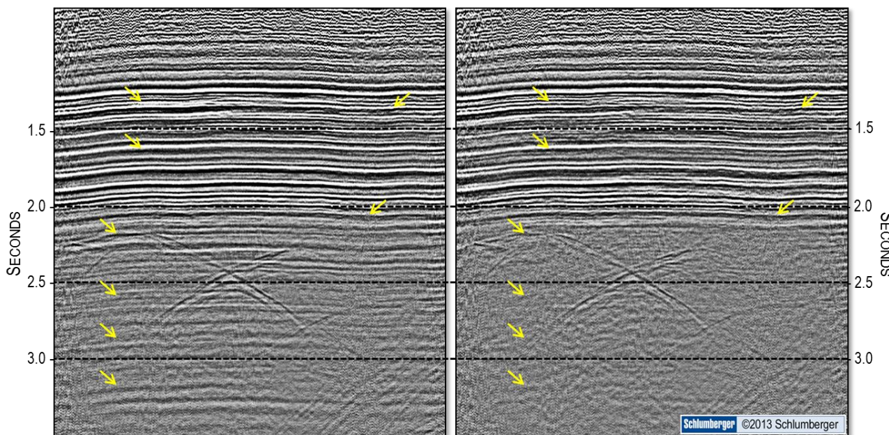
Figure 4 – Crossline stacked section before (left) and after (right) the multiple attenuation. Arrows show the data set improvement after applying the workflow.
