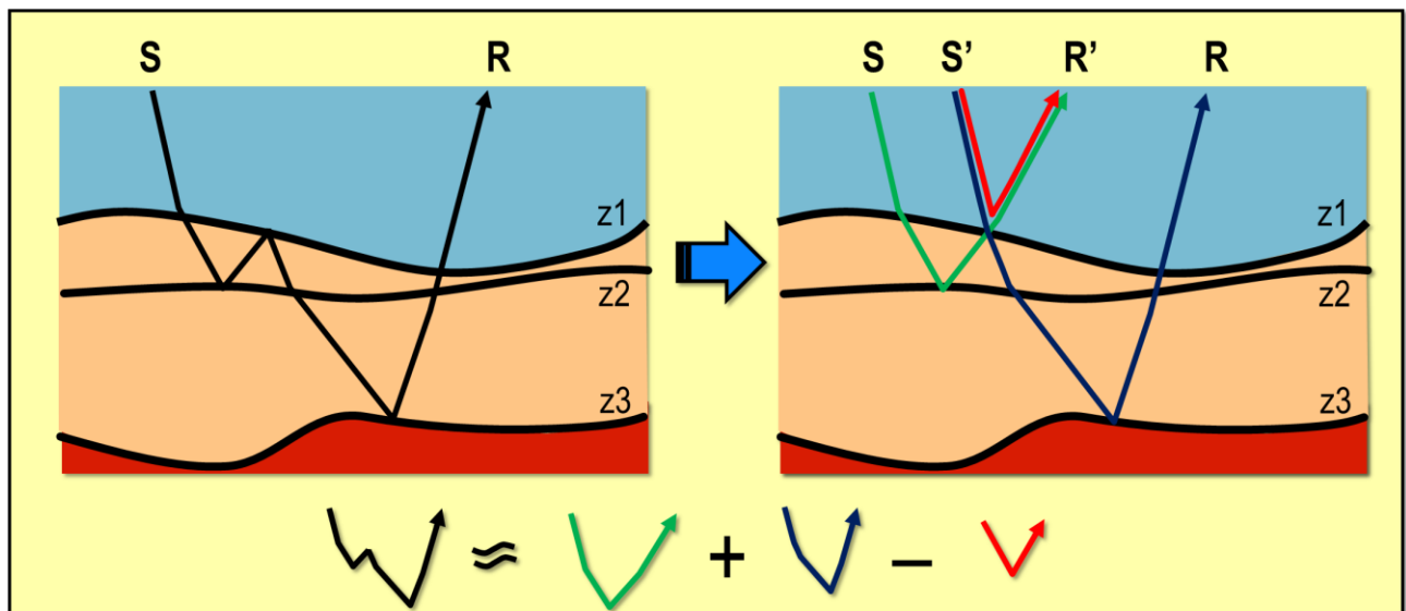
Figure 1 – A given internal multiple (left) can have the traveltimes constructed using three primary events (green, blue and red) from the subsurface that satisfies the higher-lower-higher relationship of z_3 > z_2 > z_1 .
