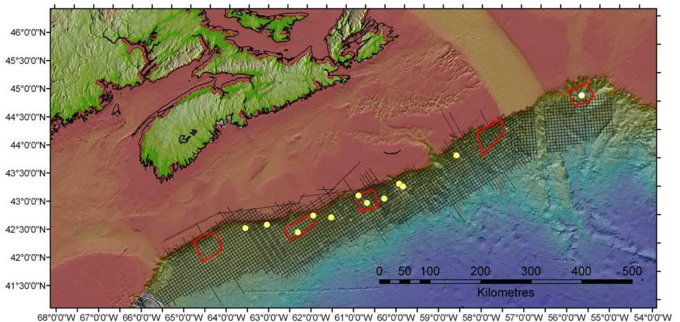
Figure 1: The modern seafloor bathymetry of the Scotian margin shows numerous canyons. Red polygons are 3D seismic volumes used in this study. Black lines are 2D seismic track lines (TGS-NOPEC). Yellow dots are exploration wells on the slope.
