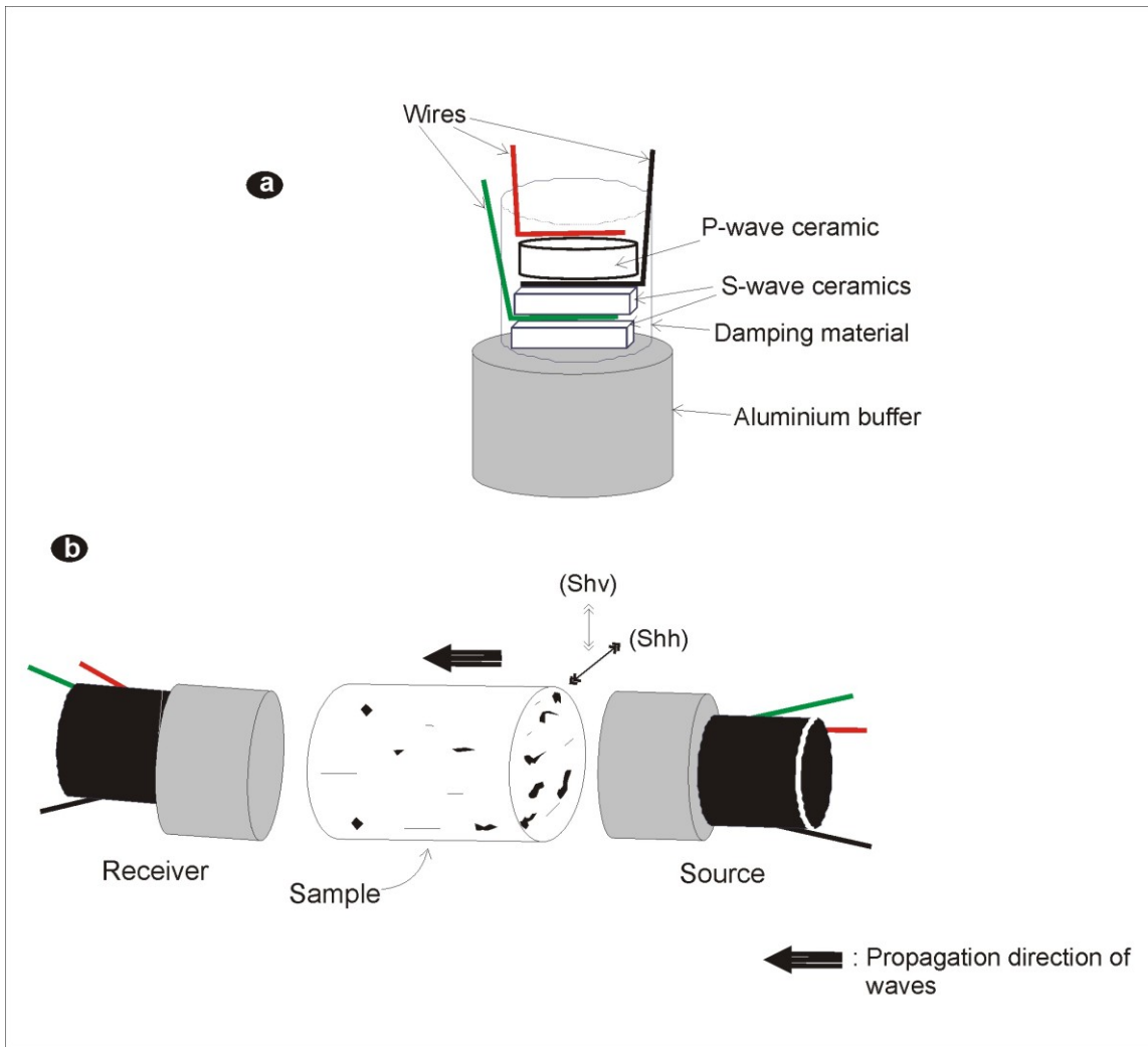
Figure 1: (a) Source/receiver transducer. (b) Assemblage Sample + Transducers. Arrow (Shh): Shear wave propagating horizontally with particles vibrating in horizontal direction (that means parallel to the rock layering); Arrow (Shv): Shear wave propagating horizontally with particles vibrating in vertical direction.
