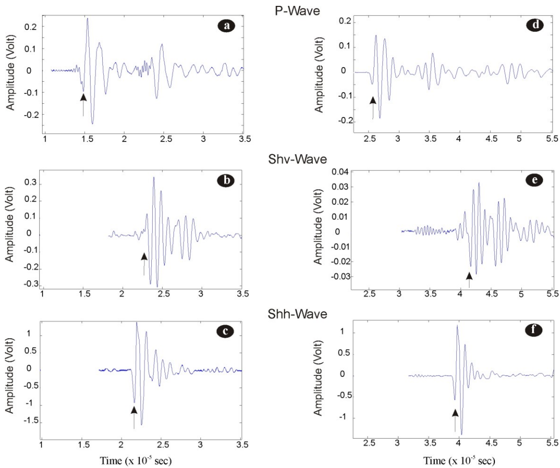
Figure 2: P- and S- waveforms under a confining pressure of 10 MPa. (a), (b), and (c): Signals through the aluminium buffer in the absence of sample. (d), (e), and (f): Signals through the buffer and the sample. The travel times is usually picked at the first extremum, marked by arrows. Shv- and Shh-waves were generated by the top and bottom S-wave ceramics in the transducer system, respectively (see figure 1a, b). The polarization axis of the bottom S-wave ceramic ( Shh-wave) was parallel to the weakly developed rock layering.
