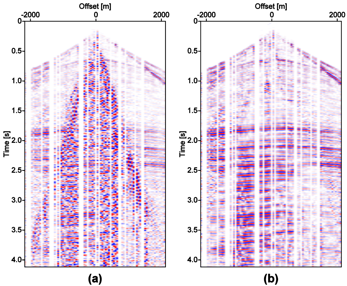
Figure 3 – (a) Randomly decimated shot gather. (b) Data in (a) cleaned by subtracting the noise model constructed using LWD. 22 out of 86 traces were muted.
