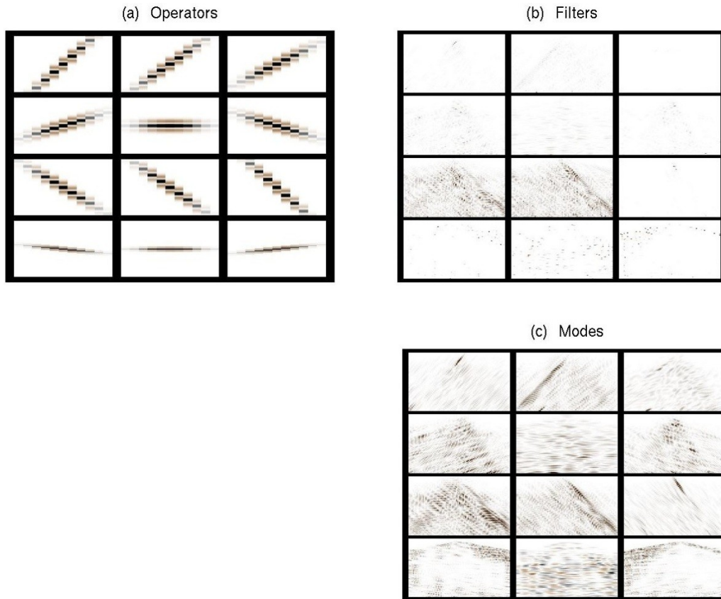
Figure 1 – (a) Compact local operators used to reconstruct the data shown in Figure 3 (a). The low frequency local operators in the top three rows of (a) model ground roll while the high frequency local operators in the bottom row model the reflections. (b) Shaping filters. Each shaping filter shapes one local operator in (a) into a mode seen in (c). The full data reconstruction is obtained by summing all the modes.
