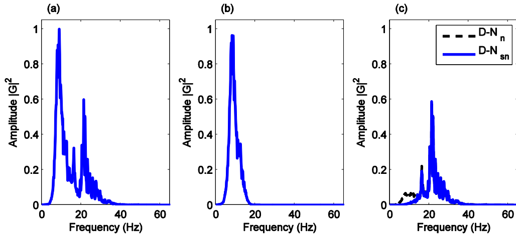
Figure 4 - (a) Amplitude spectrum of the input field data in Figure 3 (a). (b) Amplitude spectrum of ground roll model recovered by LWD, N_n . (c) Amplitude spectra of the clean data in Figure 3 (b). Noise model N_{sn} is the sum of the low pass filtered residual data and the noise model, N_n . Residual data is defined here as the data captured in neither LWD's signal nor noise model.
