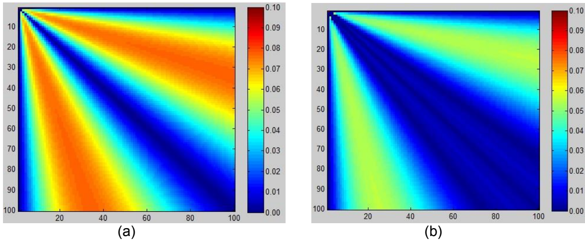
Figure 2. Error distribution (a) Vidale's result (b) adaptive stencils' result
