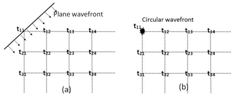
Figure 1. Illustrating (a) a plane wavefront and (b) circular wave from a point source propagating through a grid model.
