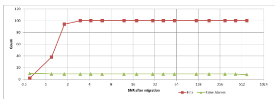
Figure 1: Count of detected events as a function of SNR after migration. Detected events matched to modeled events are shown as hits, events without a match are shown as false alarms.
