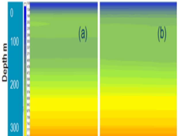
Figure 12: (a) Inversion of synthetic data from inverted model at a shot location in Figure 9. (b) Final inversion model of real data at the location.
