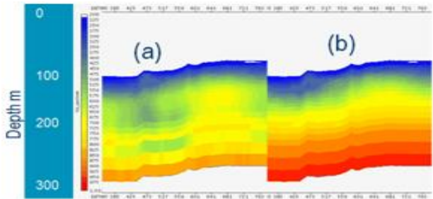
Figure 9: Depth model from pulse data for 2-20 Hz (a) and 4-20 Hz (b).
