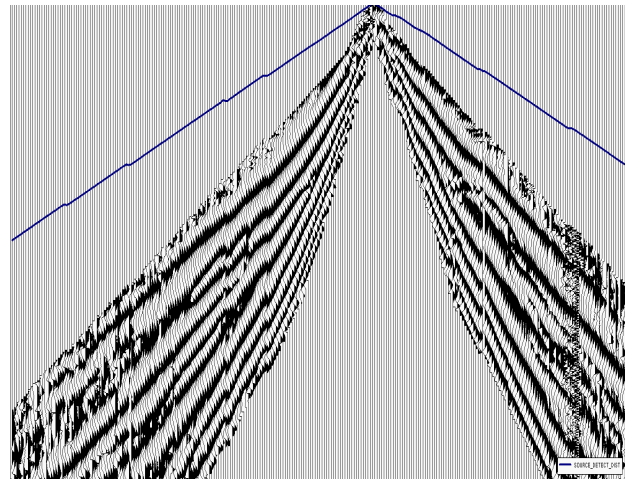
Figure 6: Processed shot gather example.
