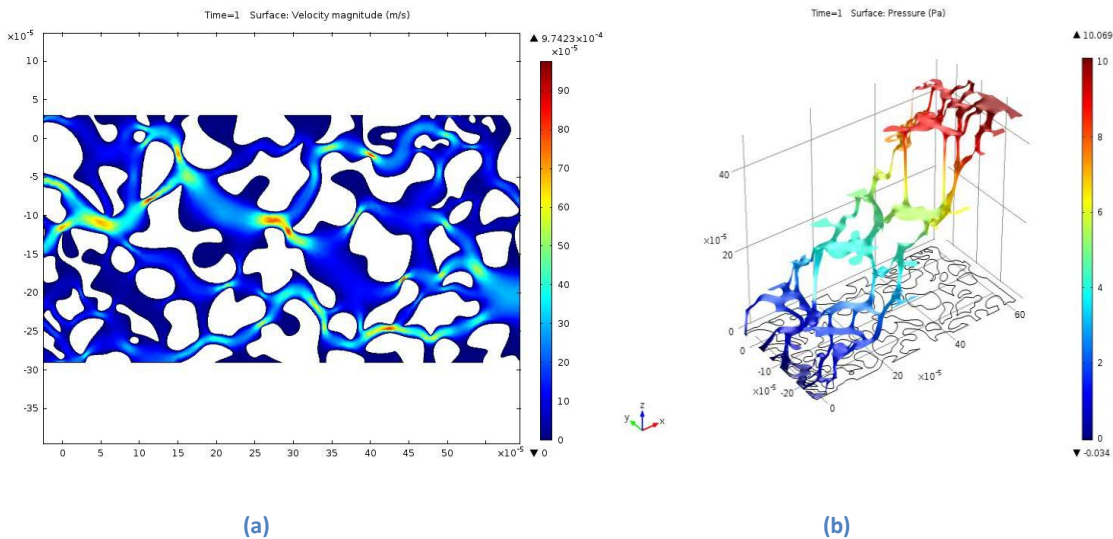
Figure 2: a) surface velocity magnitude m/s. b) surface pressure Pa
