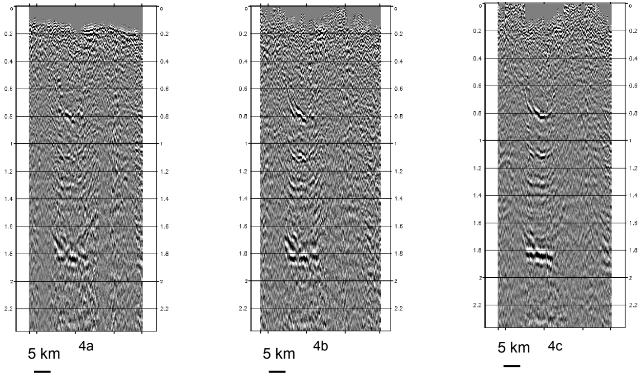
Figure 4: Psv CSP a) PP source statics b) PP source statics and conventional PSv receiver statics c) PP source statics Monte-Carlo approach PSv receiver statics
