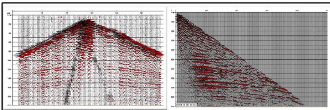
FIG. 2. Two-side CMP gather to the left and one side CSP gather to the right at the same location. Taken from Guirigay et al. 2011.
