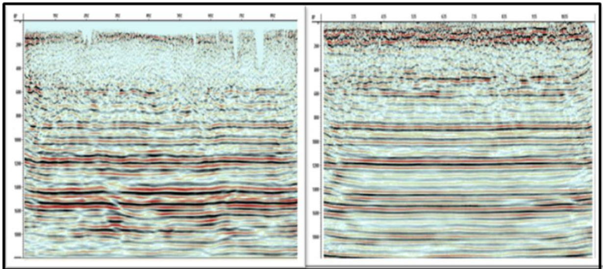
FIG. 4. Kirchhoff poststack migration (left) and EOM stacked section using a V(t) (right)
