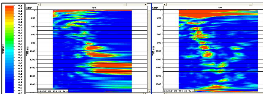
FIG. 3. Semblance display for a CMP (left) and a CSP gather (right) at the same location
