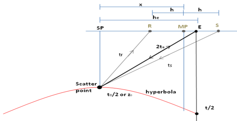
FIG. 1. Geometry of Kirchhoff prestack time migration with source S and receiver R. and equivalent offset h_e . Taken and modified from Bancroft et al. 1998.
