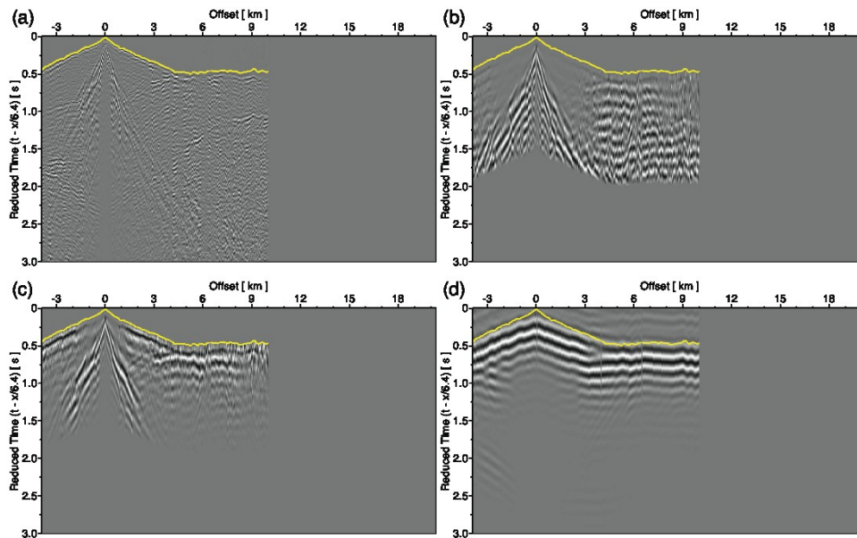
Figure 1: (a) Shot gather from a long-offset seismic line acquired in the Foothills, after (b) bandpass filtering to 8 Hz and time-windowing, and (c) with time-damping of \tau = 0.25 s applied. For comparison, (d), the corresponding synthetic shot gather generated in the starting velocity model, also with \tau = 0.25 s.
