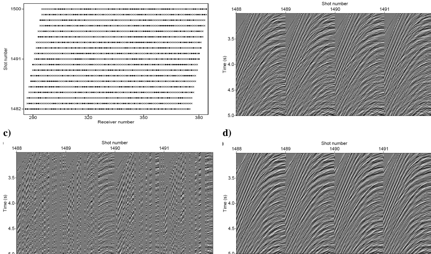
Figure 3: a) Source and receiver positions of the data from the Gulf of Mexico. Filled circles show the available traces and crosses show the missing traces. b) Original data. c) Section of missing data. d) Reconstructed data using the proposed method.
