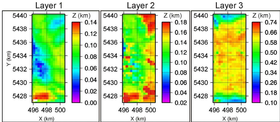
Figure 2: Depths to the bases of the three layers in the starting model for refraction statics inversion. Layer velocities are 0.67, 1.5, and 2.0 km/s, respectively, over a half-space of 3.0 km/s.
