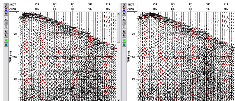
Figure 4. Acceleration domain receiver gathers, NMO corrected, with a 20 Hz lowcut for display. Left: Geophone. Right: DSU.
