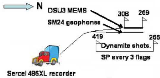
Figure 2: Geometry of the dynamite shot comparison at Spring Coulee, Alberta.
