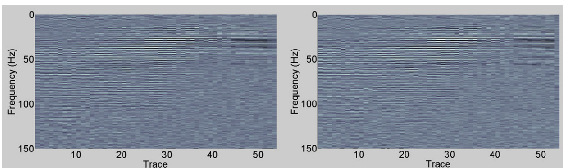
Figure 8. FX phase coherency, average of all receiver gathers. Left: Geophone. Right: DSU.
