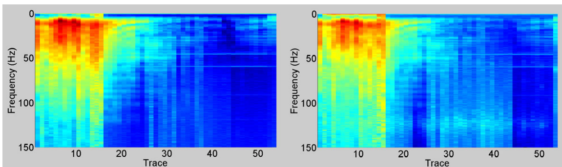
Figure 7. FX amplitude, average of all receiver gathers, dB scale. Left: Geophone. Right: DSU.
