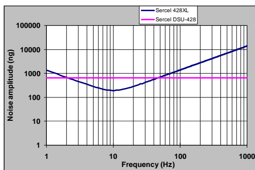
Figure 1: Modeled noise floor of a geophone and DSU recorded with the Sercel 428XL system, based published specifications of the DSU-428, the 428XL recording system and the SM24 geophone element.
