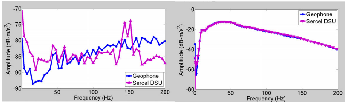
Figure 4. Acceleration amplitude spectra. Left: Noise before first breaks. Right: Average of all traces (0-4 sec).
