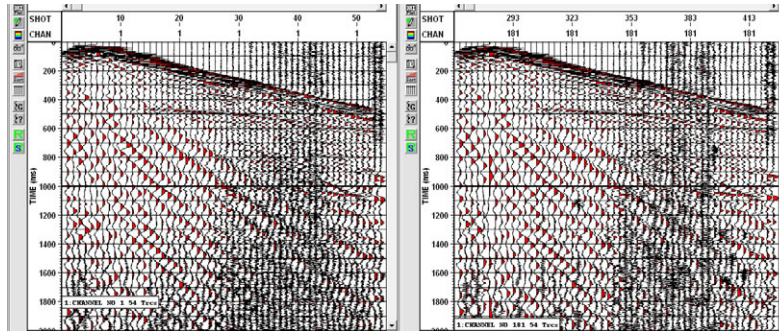
Figure 3. Acceleration domain receiver gathers. Left: Geophone. Right: DSU.
