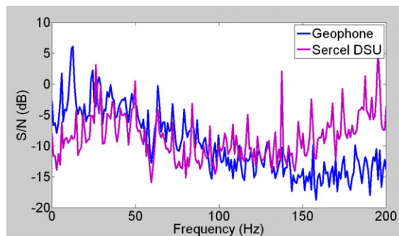
Figure 5. Acceleration domain spectra, noise before first breaks.
