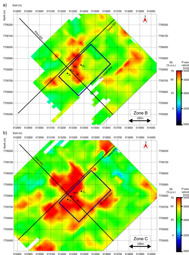
Figure 4 (RIGHT): Velocity map inferring extent of gas hydrate zones B (top) and C (bottom). Color code shows P-wave velocity in m/s and gas hydrate concentration in % of pore space (% p.s.).
