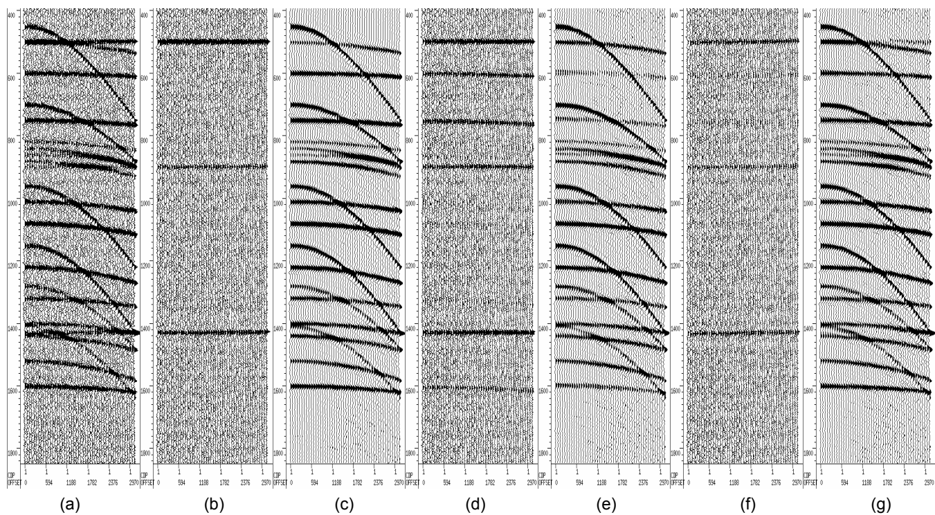
Figure 4: Synthetic data (noise model B): the same as Figure 2 (model B), but strong random noise is added.
