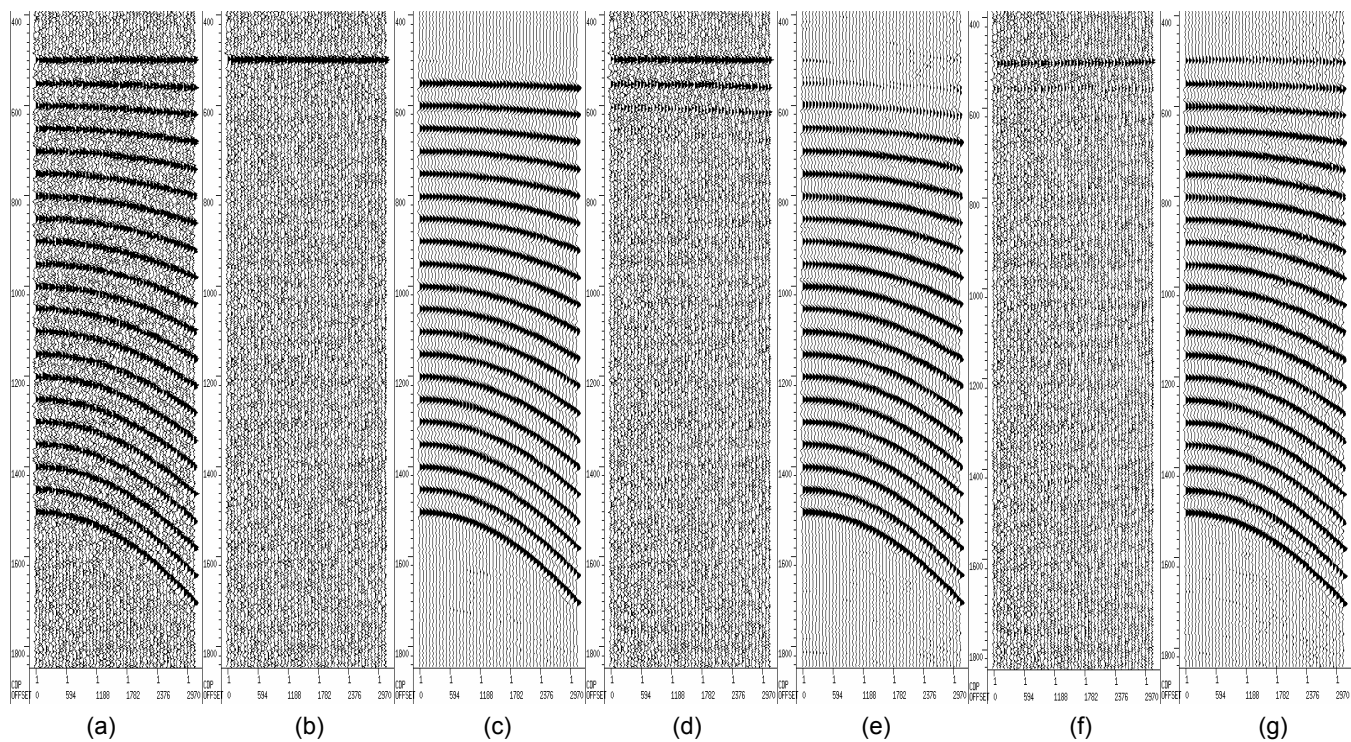
Figure 3: Synthetic data (noise model A): the same as Figure 1 (model A), but strong random noise is added.
