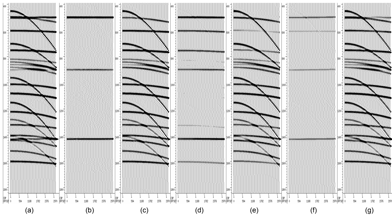
Figure 2: Synthetic data (model B): twenty five events, three primaries and twenty two multiples with different curvatures: moveouts at far offset are 10, 15, 18, 25X3, 30X2, 35X2, 40, 45, 50X2, 60X2, 180, 200, 225, 260, 280, 300 ms (a). The results of multiple attenuation using (b) MIDAS; (d) HRR with removing from moveout 20ms; (f) HRR from moveout 4ms. Corresponding removed multiples are shown in (c), (e) and (g) respectively.
