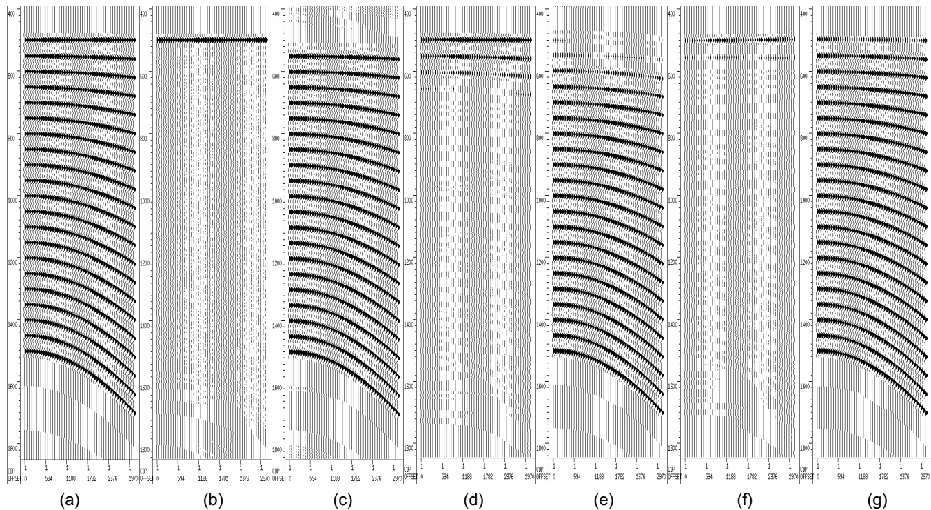
Figure 1: Synthetic data (model A): twenty one events, one primary and twenty multiples with different curvatures: moveouts at far offset distributed evenly from 10 ms to 200 ms (a). The results of multiple attenuation using (b) MIDAS; (d) HRR with removing from moveout 20ms; (f) HRR from moveout 4ms. Corresponding removed multiples are shown in (c), (e) and (g) respectively.
