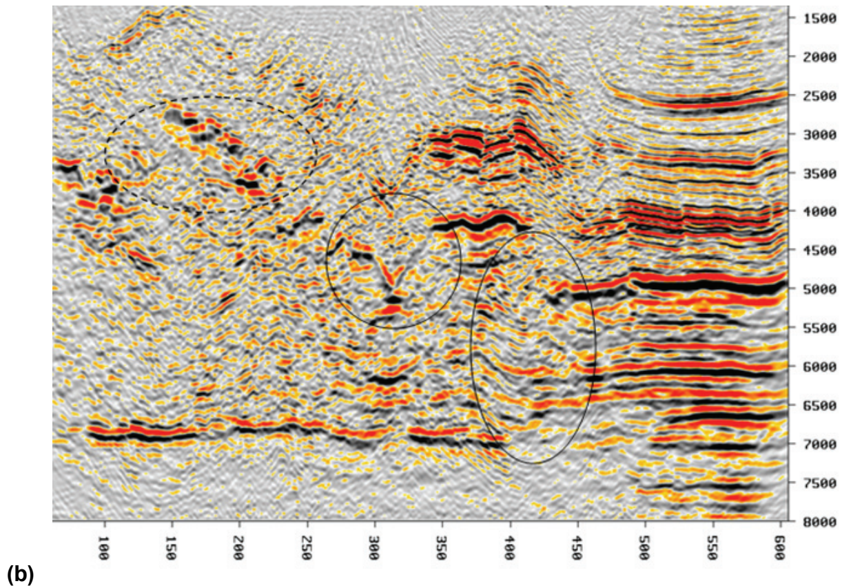
Figure 3: A cross-line from the 3-D Copton survey, showing a comparison of (a) TTI Kirchhoff migration; with (b) TTI wave-equation migration. The Kirchhoff migration included frequencies up to 80Hz, whereas the WEM was migrated up to 40Hz. Solid black ellipses indicate areas where WEM appears superior to Kirchhoff. Dashed ellipse shows an example where Kirchhoff is superior.
