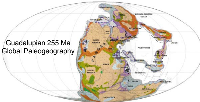
Figure 1. Representative products from our Global Atlas of Carbonate Fields. 1A. Modern-day distribution of 8276 carbonate fields. 1B. Late Permian global paleogeography with distribution of Guadalupian age carbonate reservoirs (black dots). 1C. Frequency distribution of carbonate fields by age.
