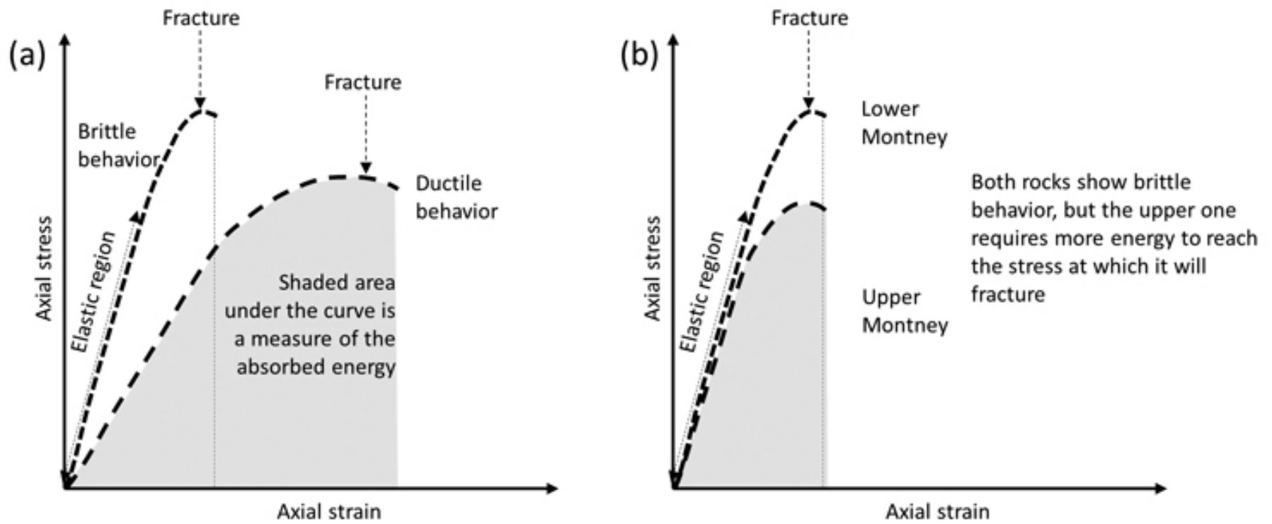
Figure 1. (a) Brittle versus ductile behavior of rock samples as seen on a stress-strain graph. (b) Both rocks showing brittle behavior, but one requires more energy to reach the stress level at which it will fracture.
