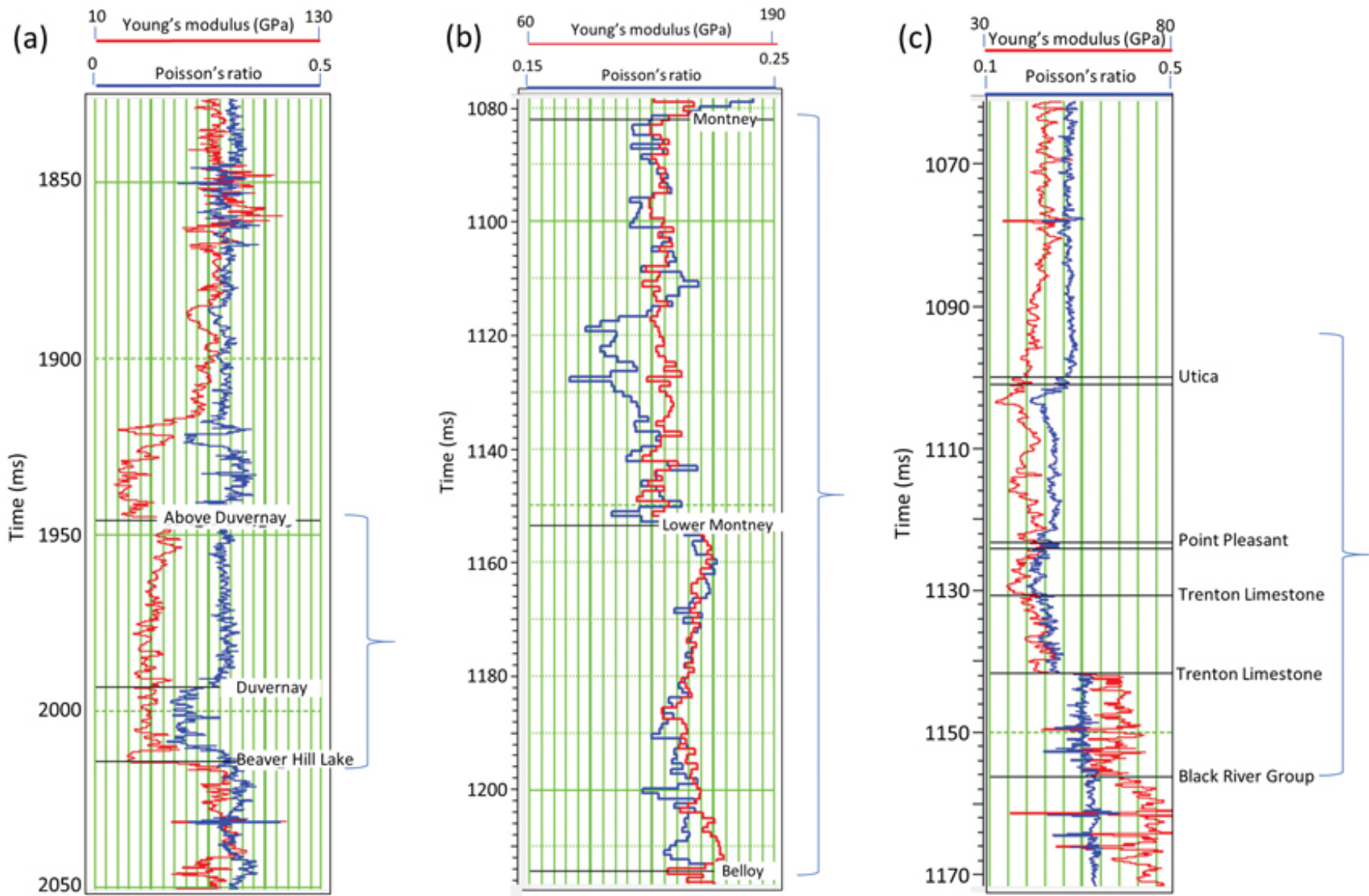
Figure 2. Shows the Young's modulus and Poisson's ratio curves for well data from (a) Duvernay Shale in Kaybob area in central Alberta, Canada, (b) Montney Shale in British Columbia, Canada, and (c) Utica Shale from eastern Ohio, USA. Notice a crossover between them only for Upper Montney. Such a crossover is not seen for the Duvernay and Utica shale intervals.
