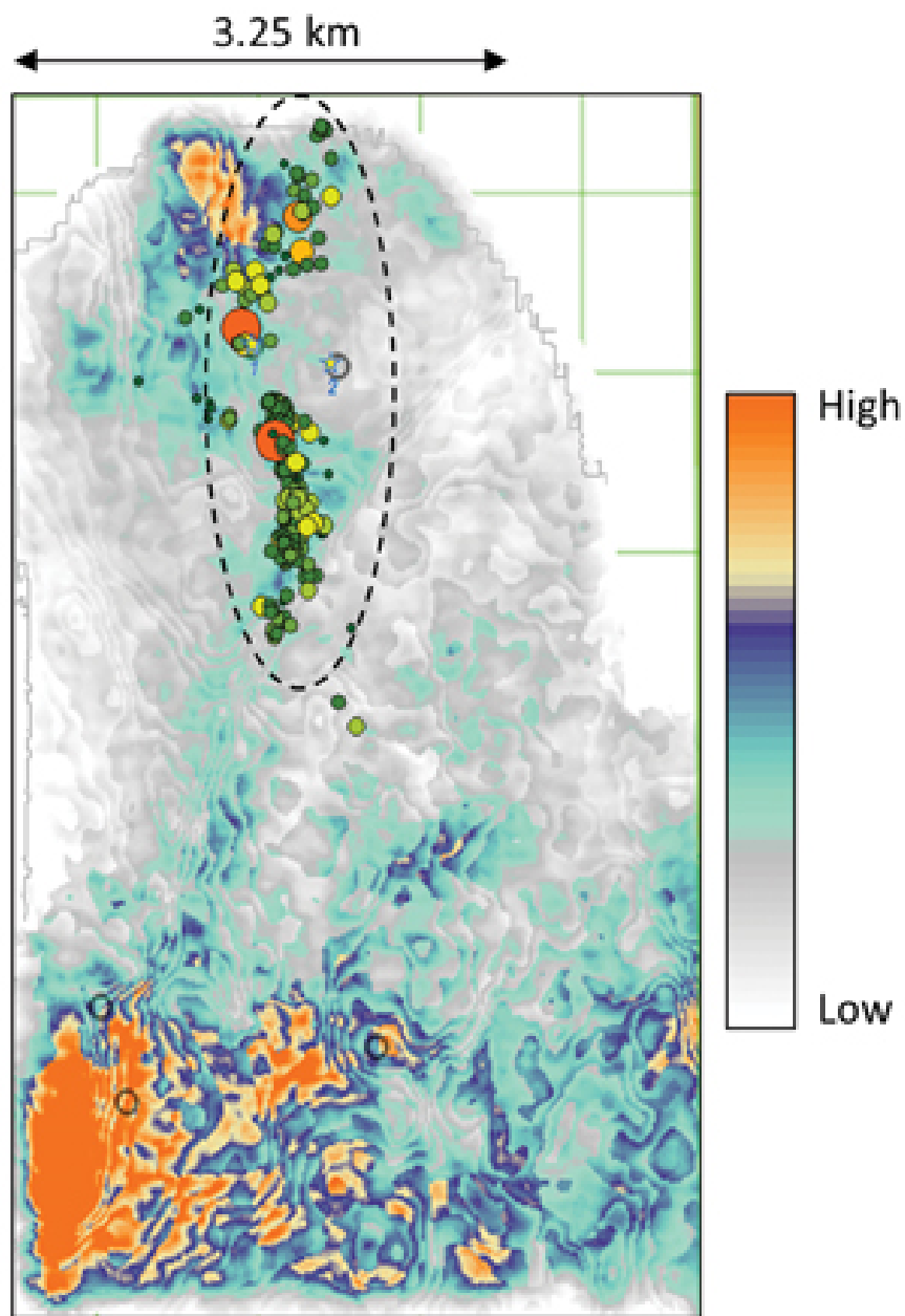
Figure 4. Horizon slice from inverse fracture toughness measure volume for the Duvernay Formation in the Fox Creek area in central Alberta, Canada. Notice, the high values of inverse fracture toughness measure (or low values of fracture toughness measure) correlate well with the induced seismicity data overlaid on the display. Induced seismicity data is courtesy of Repsol Oil and Gas, Canada.
