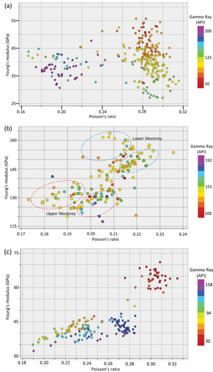
Figure 3. The crossplots between Young's modulus and Poisson's ratio for well data shown in Figure 2 are shown here in Figure 3. The cluster points are all colour-coded with Gamma Ray values. Notice, the cluster points corresponding to the shale intervals of interest exhibit different values of Young's modulus and Poisson's ratio.
