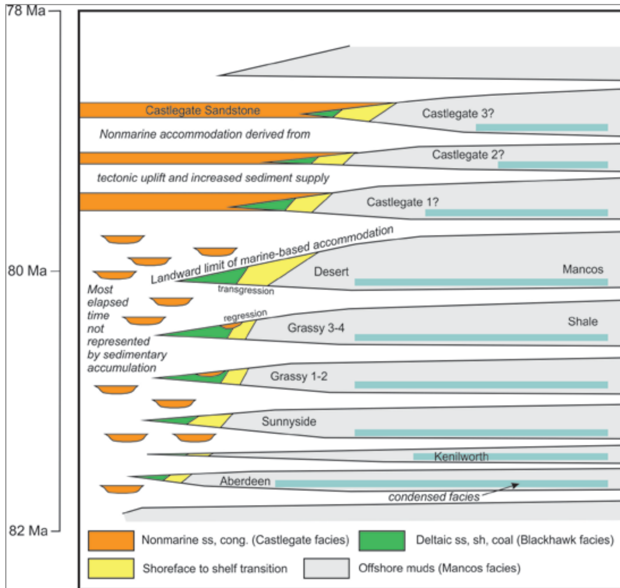
Figure 4. An interpretation of the chronostratigraphy of the Mesaverde Group. Age information is from Hampson (2010) and Seymour and Fielding (2013).
