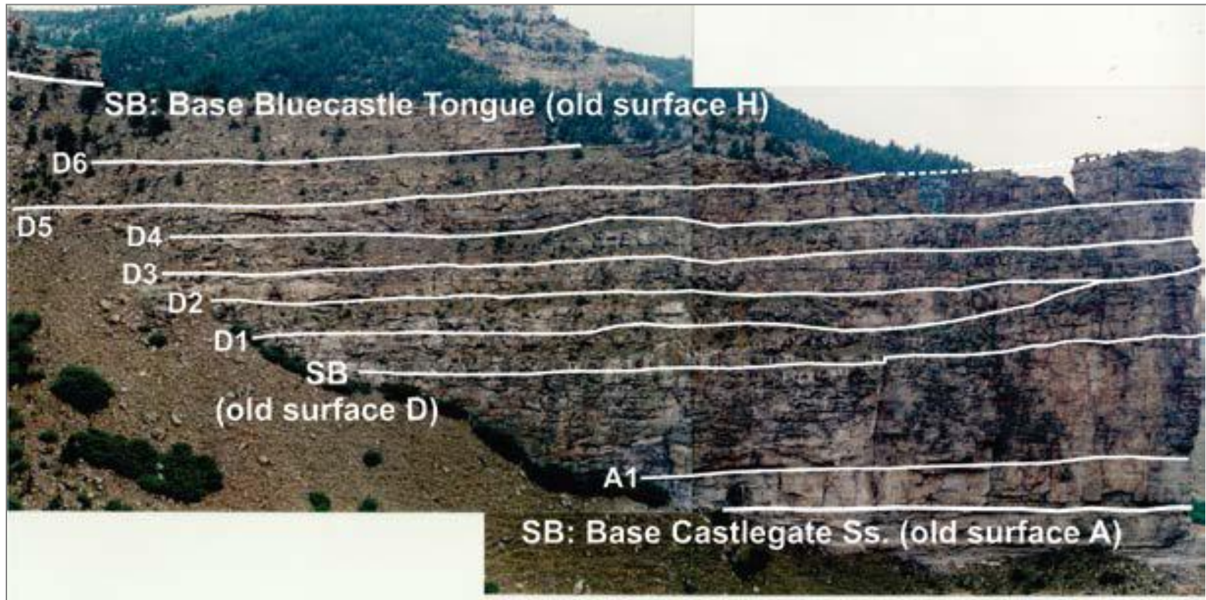
Figure 7. The type section of the Castlegate Sandstone, with key bounding surfaces. Surface D of Miall and Arush (2001a). is tentatively identified as a major intraformational unconformity and sequence boundary. Width of field of view about 250 m.
