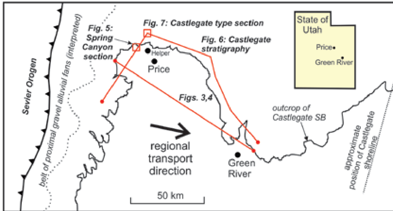
Figure 2. Location of study area, showing the locations of detailed sections and other illustrations.
