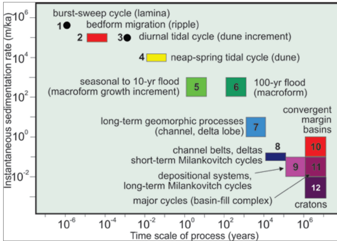
Figure 1. Rates and durations of sedimentary processes. Numerals refer to the Sedimentation Rate Scale of Miall (2013a).
