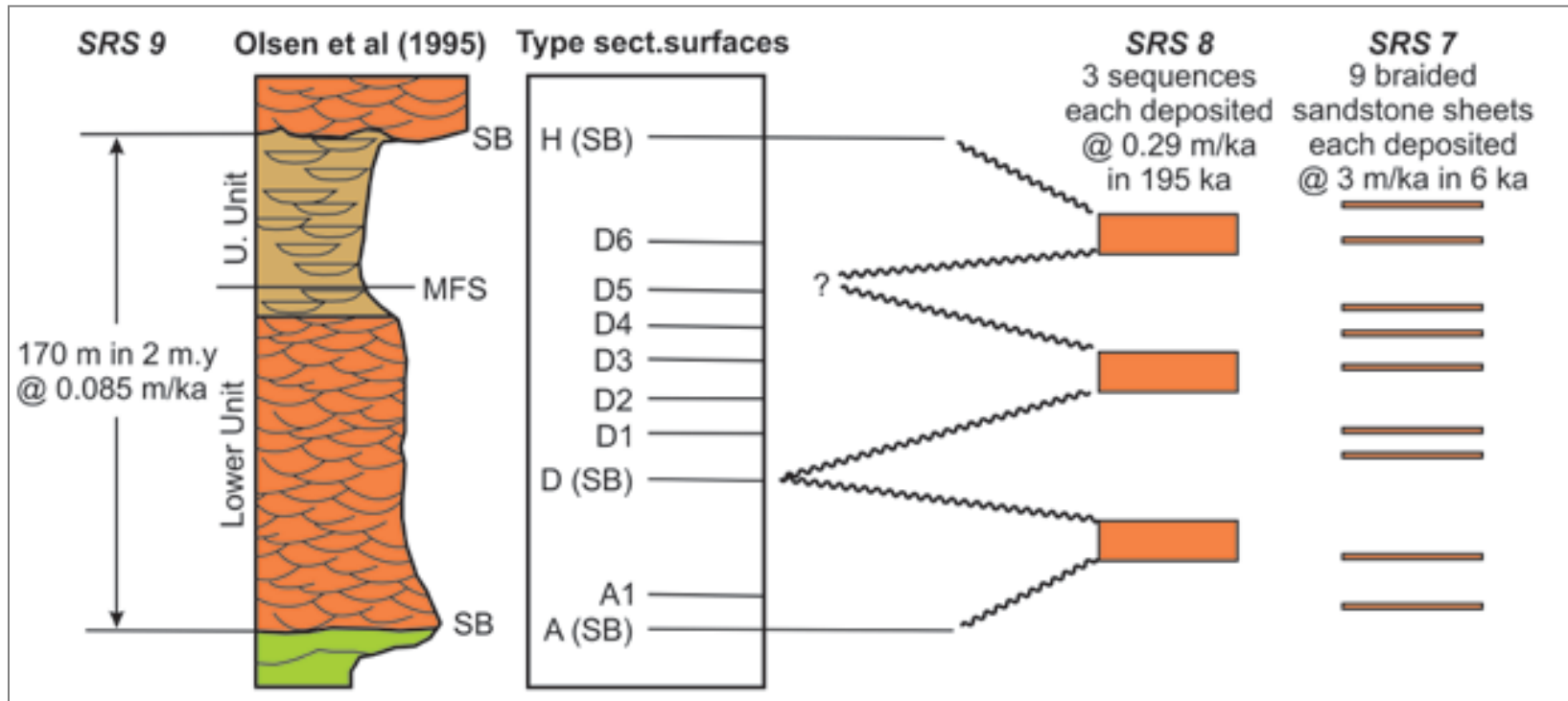
Figure 8. Different interpretations of the Castlegate Sandstone at the type section. See text for explanation.
