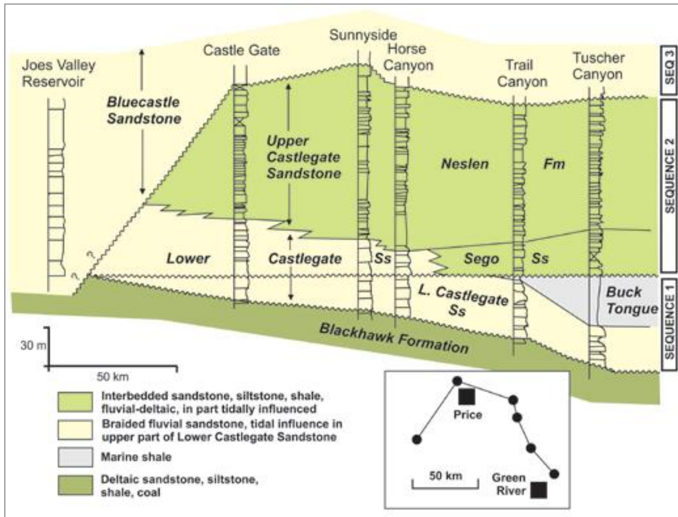
Figure 6. Stratigraphy of the Castlegate Sandstone (from Miall and Arush, 2001a; based on Willis, 2000 and Yoshida, 2000).
