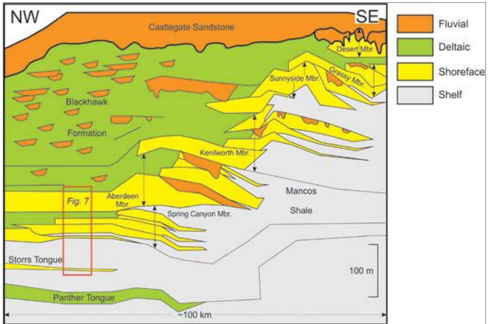
Figure 3. Regional cross-section of the Mesaverde Group; adapted from Seymour and Fielding (2013), after the detailed mapping of Young (1955).
