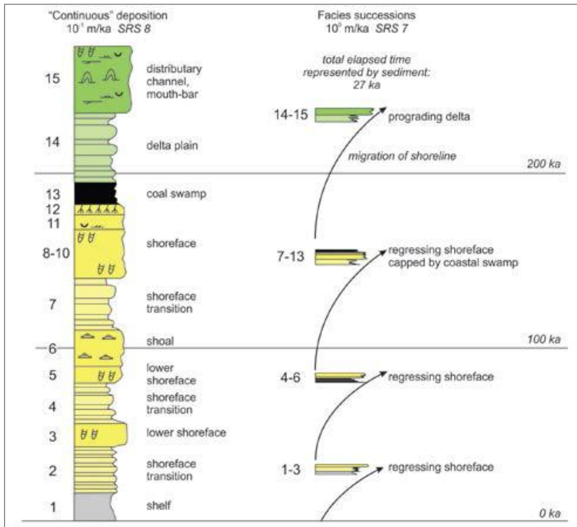
Figure 5. The Spring Canyon Member dismembered. Fifteen numbered lithofacies units are present. At left, the section is plotted to correspond to a SRS 8 time scale, suggesting an approximate 273 ka timespan for the accumulation of the succession. At right, the same section is evaluated in terms of an SRS 7 time scale, for which sedimentation rates are an order of magnitude more rapid. The section is subdivided into a set of progradational coastal plain and shoreface successions (original section from Cole and Friberg, 1989).
