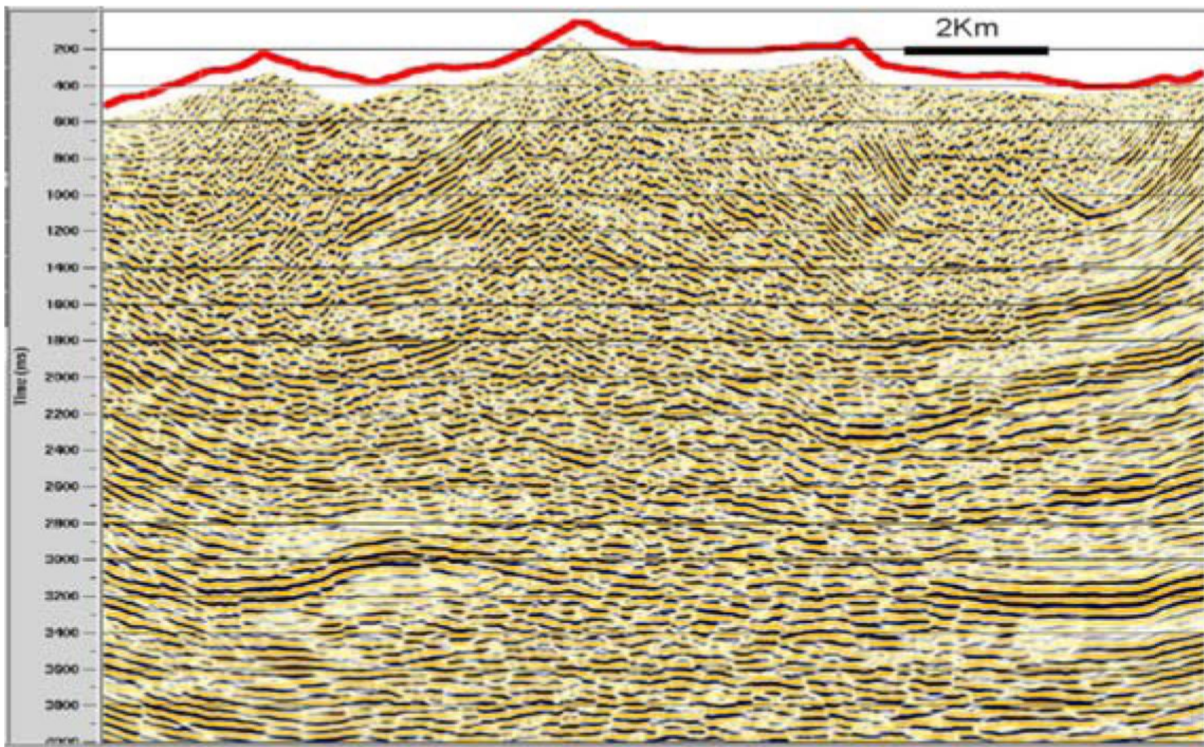
Figure 4. Final PSTM stacked section (red line indicates the elevation in time domain).
