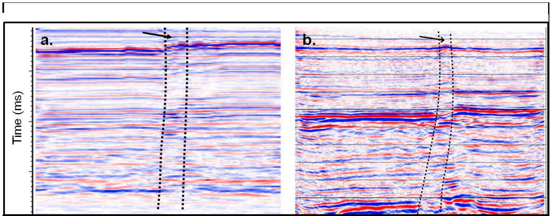
Figure 5. Post-stack migrated seismic sections imaging a fault rupturing the surface for a) the physical model b) the Greendale fault zone, New Zealand. The deformed fault zone is outlined.
