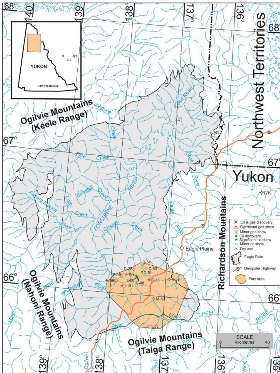
Figure 1. Chance sandstone stratigraphic gas play.
