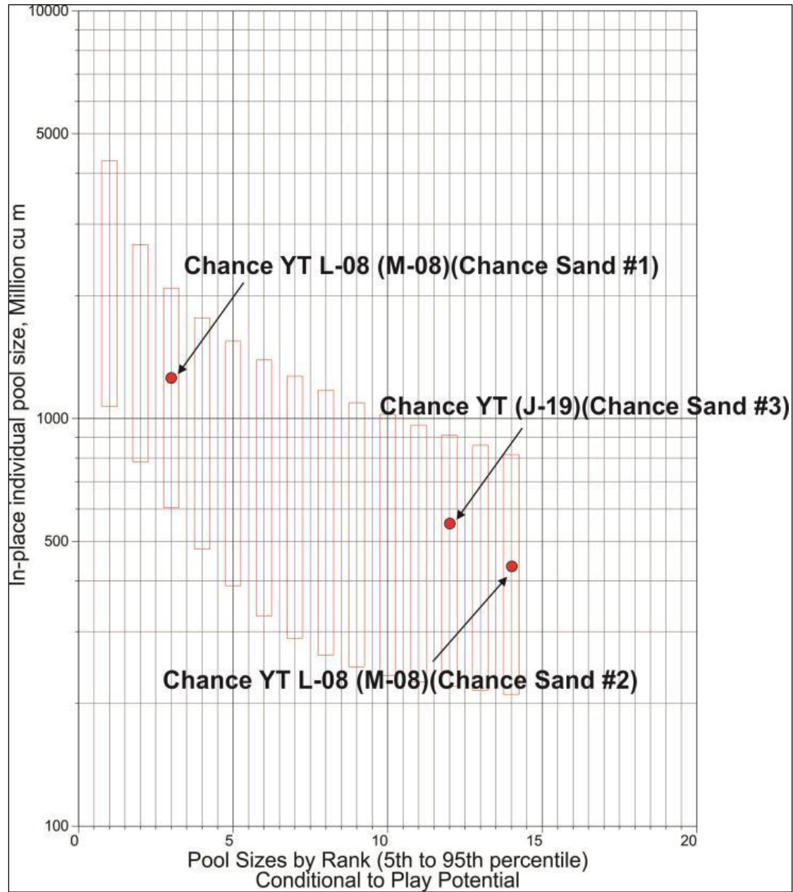
Figure 2. Pool-size-by-rank plot of the Chance sandstone stratigraphic gas play, Eagle Plain.
