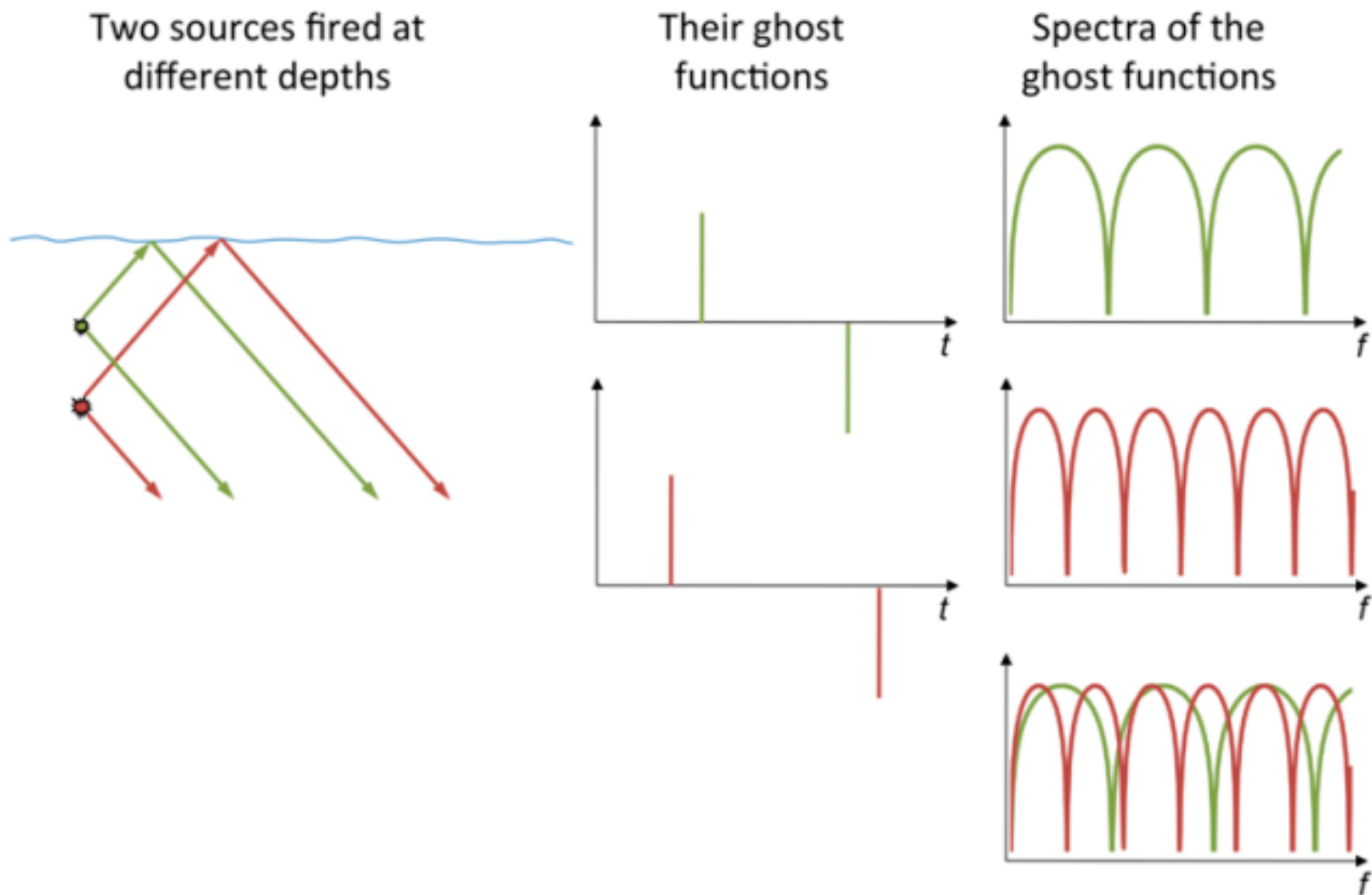
Figure 3. Illustration of the time and depth distributed source. The depths are chosen such that the independent depths exhibit complementary ghost functions – so where one source depth has a notch, the other has strong signal and vice versa.
