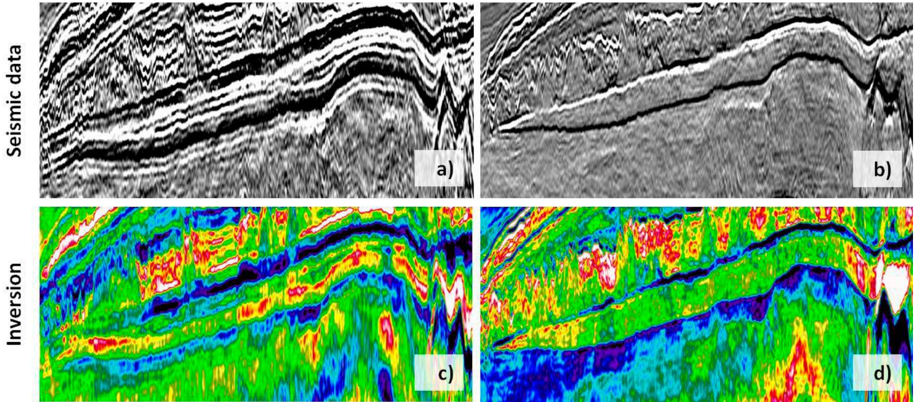
Figure 6. Comparison of a conventional dataset (a) with a ghost free dataset (b). The two datasets have been inverted below and simple comparison between c) and d) reveals how much better the broadband ghost free data is. Extremely thin layers can now be characterized using the new ghost free broadband data.
