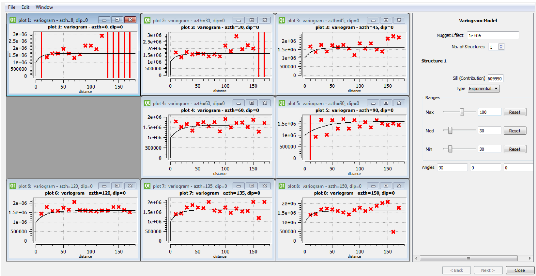
Figure 2. Screen capture of the experimental and modelled variograms from the Grignantes outcrop (SGeMS software).
