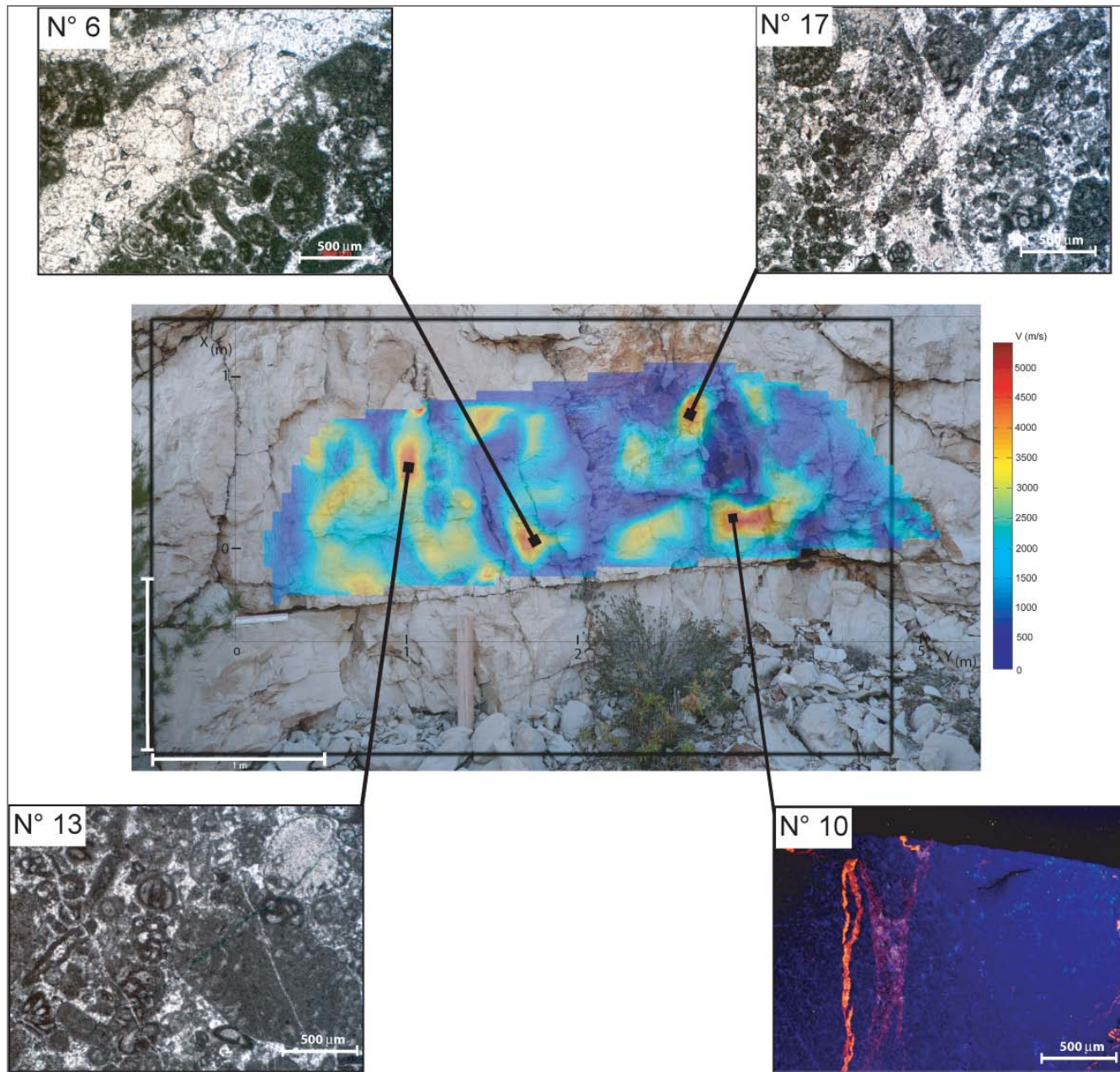
Figure 1. Map of variations of P-wave velocity measured on the Cassis outcrop. Microphotographs are from thin sections sampled on the high V_p spots and present numerous cemented cracks (photo of thin section N°10 was made using cathodoluminescence).
