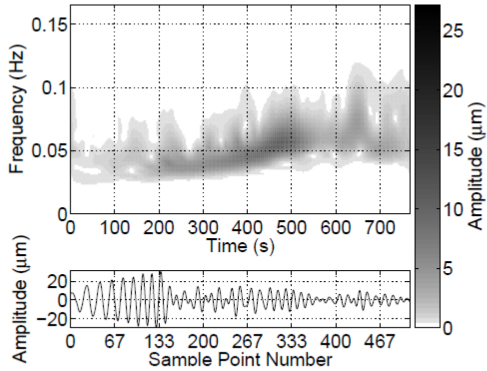
Figure 6. TFR of semi minor axis.
