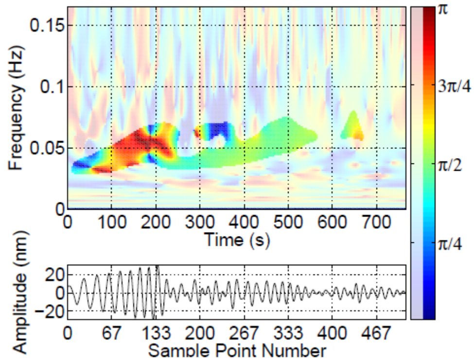
Figure 7. TFR of ellipse plane dip.
