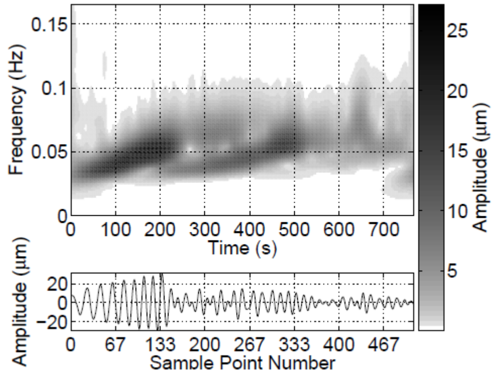
Figure 5. TFR of semi major axis.
