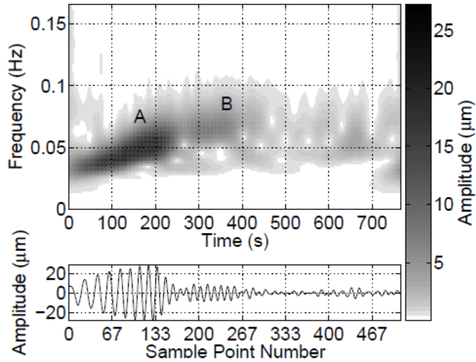
Figure 3. TFR of transverse component.
