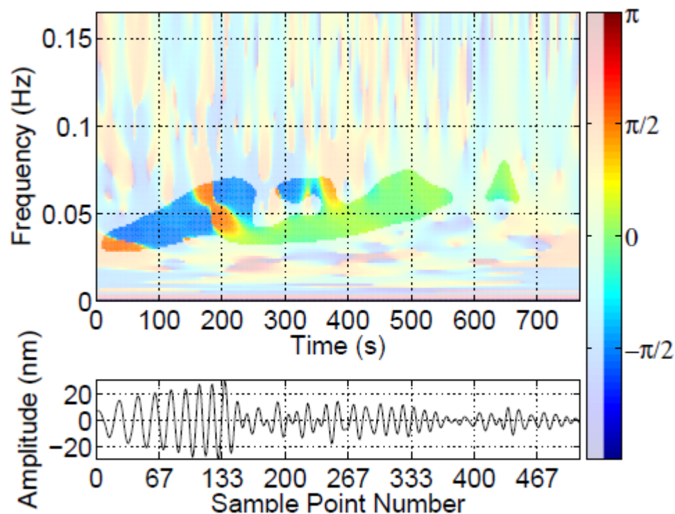
Figure 8. TFR of ellipse plane strike.
