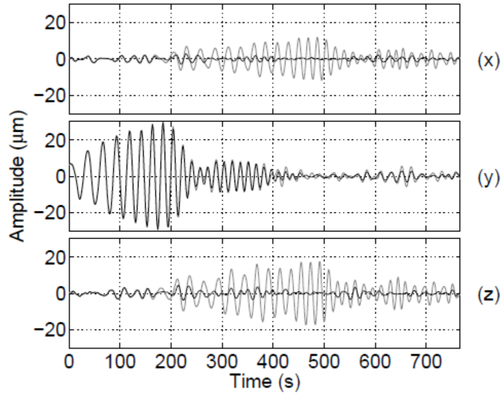
Figure 9. Filtered seismogram.
