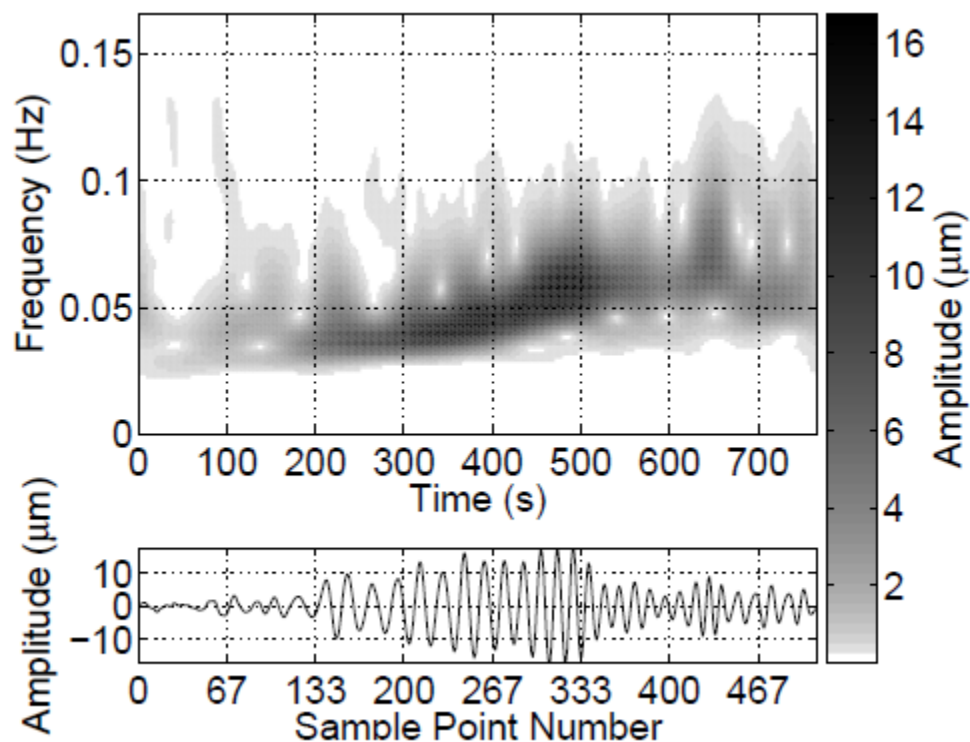
Figure 4. TFR of vertical component.
