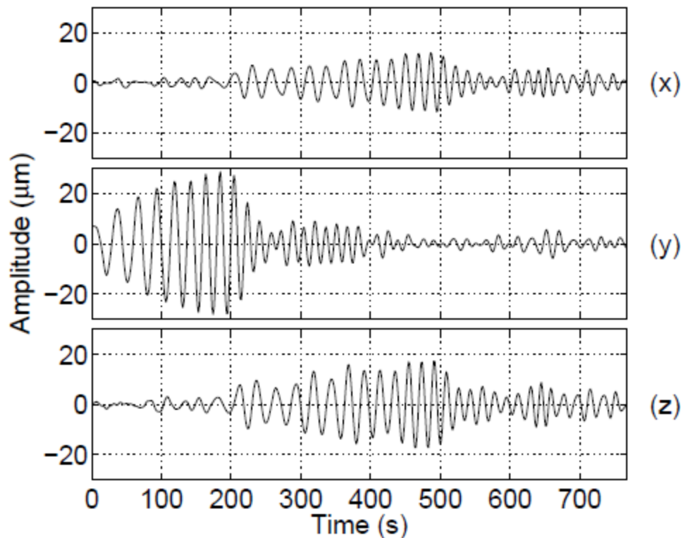
Figure 1. Earthquake seismogram.
