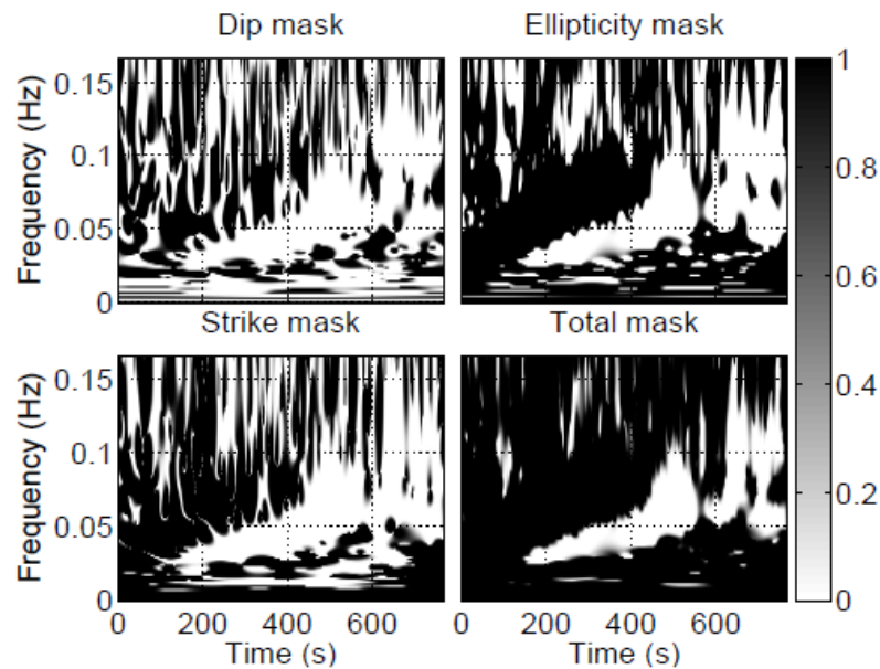
Figure 10. Masking function.
