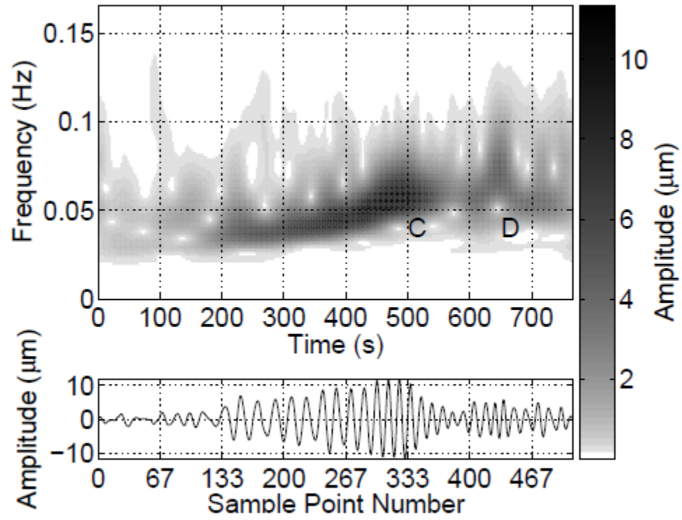
Figure 2. TFR of radial component.
