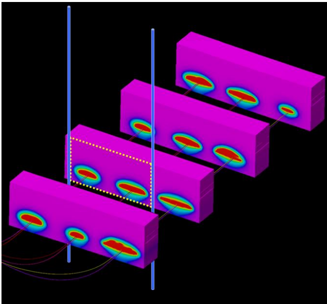
Figure 1: Cross-well experiment layout. Two vertical observation wells (blue) were planned drilled straddling two horizontal production/injection pairs. Distance between producers is 100 meters, while the distance between the observation wells is 150 meters. Color scale represents increasing temperatures during SAGD, warm colors are high temperatures.
