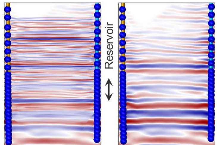
Figure 4 (above): Seismic cross-well section (left) and corresponding section from the 3D VSP baseline acquisition (right). The reservoir interval is approximately 40 m. The two observation wells and permanent three-component geophones can be found along the edges of the two sections.
