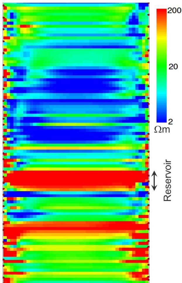
Figure 3 (left): ERT baseline image between the two observation wells. Color scale is in \Omega\text{m} , varying from high (oil sand reservoir and parts of Devonian) to low (mainly water-filled sandstone). Red circles along edges represent ERT electrode locations. The 2D section is 150 m wide and covers a depth interval of approximately 420 m. Noise along well bores is probably due to minor electrical leakages caused by imperfections in the insulation material.
