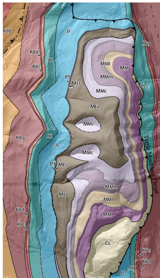
Figure 2: Hill-shaded map with unit boundaries and thrust. Scale 1:50,000.
