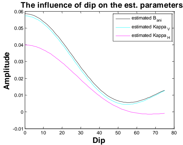
Figure 2: Inversion estimates of B_{ani} , \kappa_V and \kappa_H assuming the fractures are vertical. The horizontal axis displays the actual dip of the fractures. When the dip is 0 degrees from the vertical the estimate corresponds to the ideal solution. Non-zero dip introduces bias into the estimates (compared to ideal solution on the y-axis).
