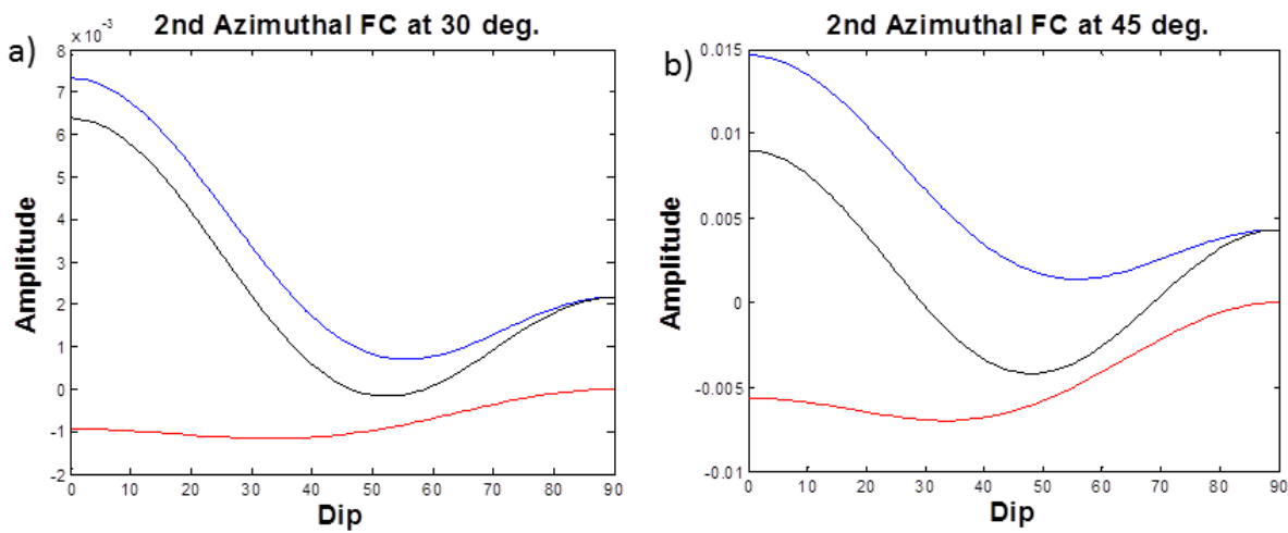
Figure 1: The effect of dip on the 2 nd FC at 30 degrees (a) and 45 degrees (b) incidence angle. The blue curve shows the contribution of the w_{12} term while the red curve shows the contribution of the w_{22} term. The total or combined response is shown in black. For small angles (i.e. 30 degrees) the w_{12} term dominates.
