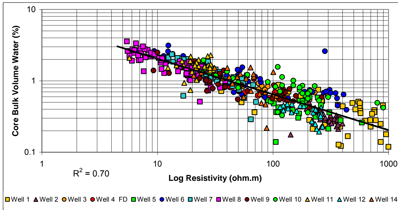
Figure 3: Montney deep resistivity-bulk volume water scatter chart
