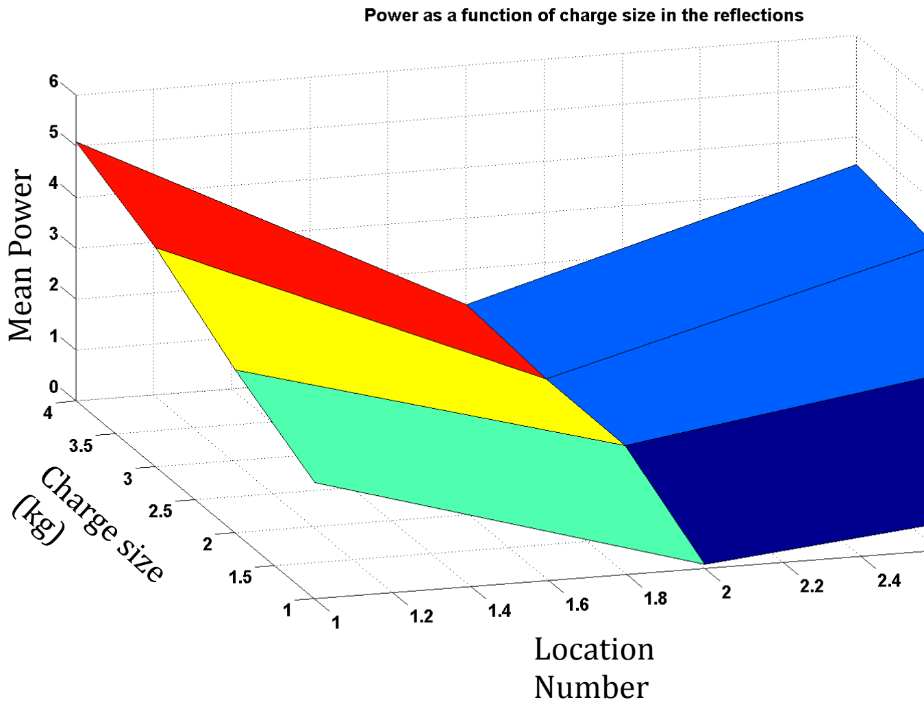
Figure 3: Mean power for the reflections resulting from different charge sizes at each location.
