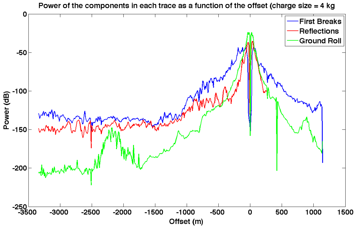
Figure 4: Power variation as a function of offset for a 4 kg test charge at location 1.
