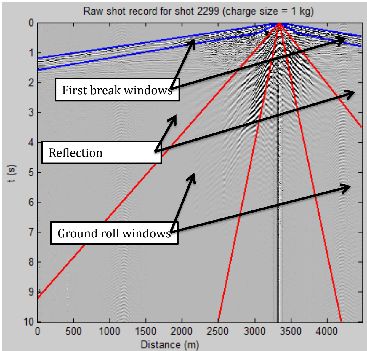
Figure 1: Time windows used to isolate each component of the shot record.
