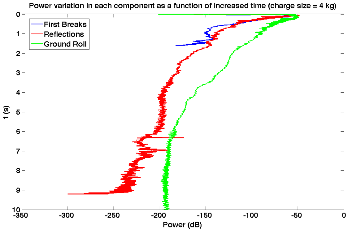
Figure 5: Power variation as a function of time for a 4 kg test charge at location 1.
