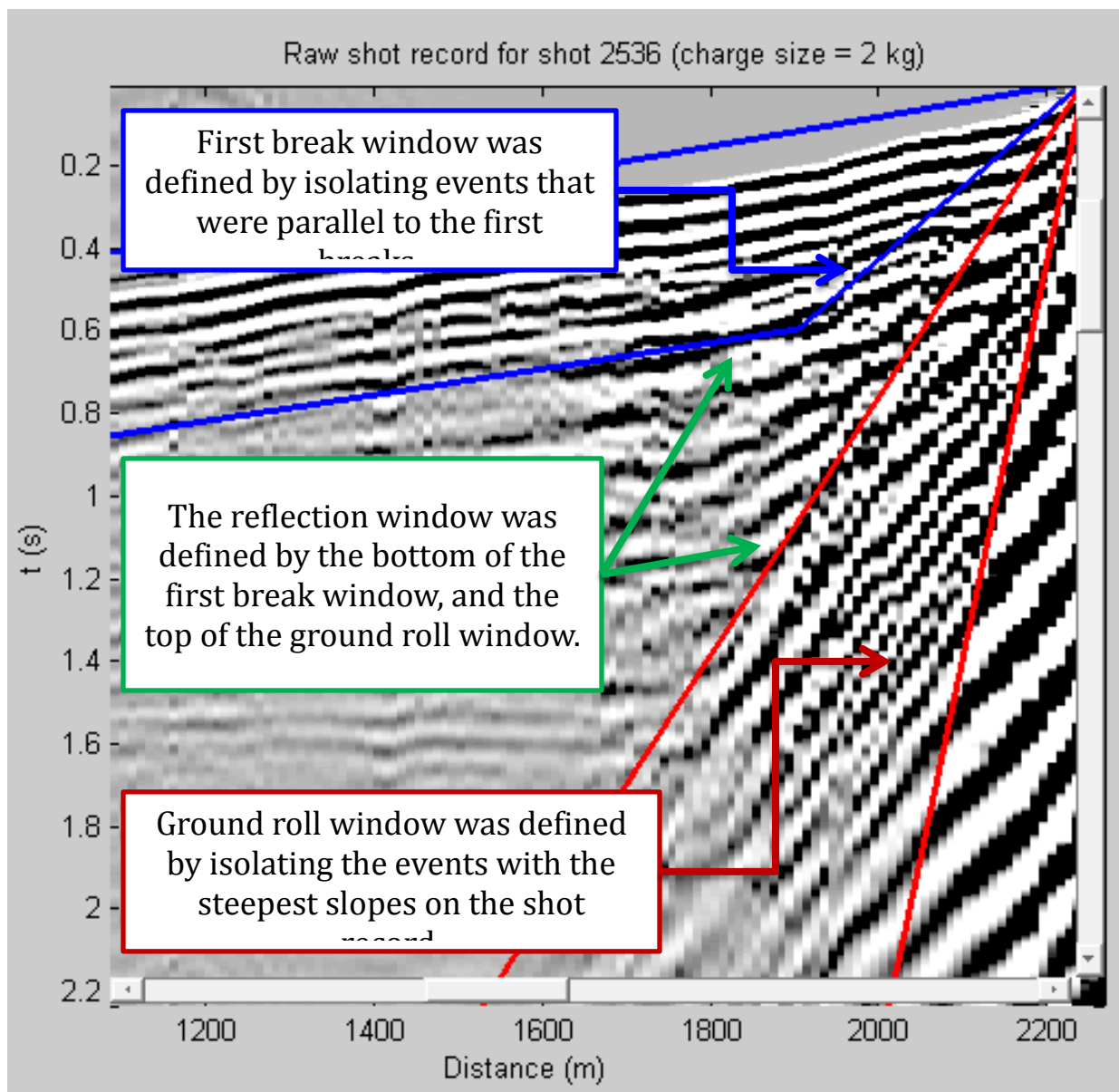
Figure 2: Criterion used to isolate each component from the rest of the shot record.
