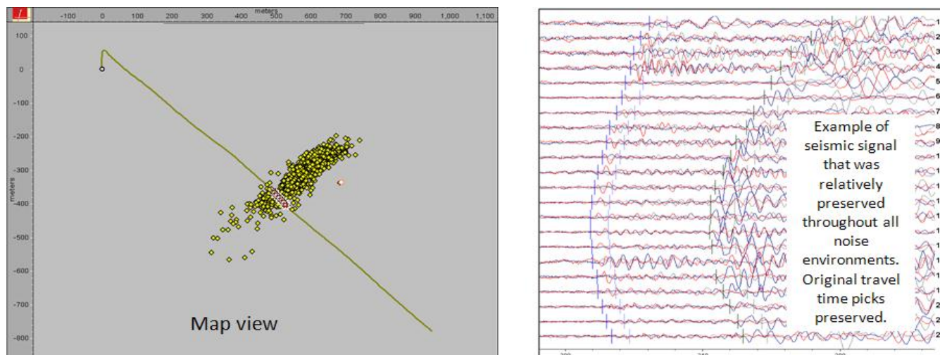
Figure 2: Microseismic mapping results based on a low noise environment (left panel) and waveform example (right panel) with original travel time picks preserved.
