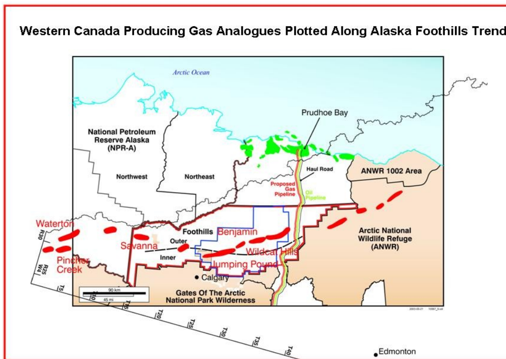
Figure 1. Scale Comparison: Alaska Inner Foothills vs. Western Canada Gas Pool (Foothills) Trend
