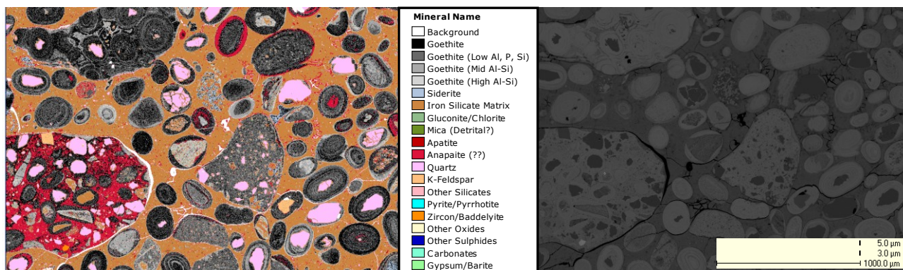
Figure 2: QEMSCAN™ false colour image (left) mapped at 5 µm and the corresponding BSE (Back Scattered Electron) Image (right) from sample R04-C1
