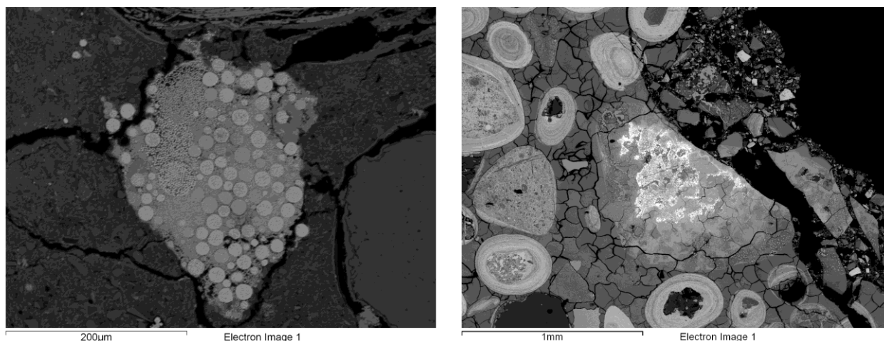
Figure 3: SEM images of framboidal pyrite (left) and a sulphide mineral (bright phase) containing nickel, cobalt, arsenic and iron.
