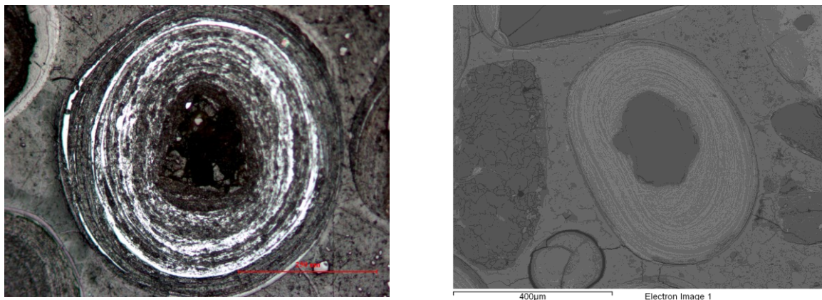
Figure 1: Left, Optical microscope photomicrograph right, a SEM image showing, both showing the layering texture of a typical ooid.
