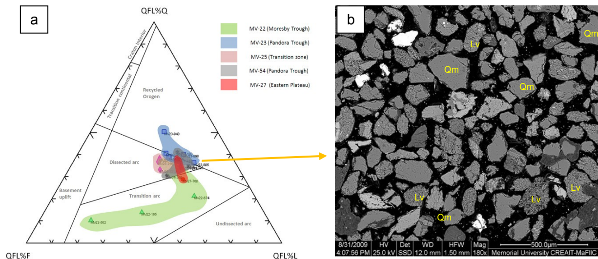
Figure 2: a) Ternary diagram using provenance fields of Gazzi-Dickinson (Ingersoll et al., 1984) showing the turbidite sources range from dissected arc to recycled orogen. b) Example of the backscatter SEM image from turbidite sand samples in core MV-23 (Pandora Trough) interval 805 cm (borderline between dissected arc and recycled orogen), showing the predominant composition of volcanic lithic (Lv) and monocrytalline Quartz (Qm).
