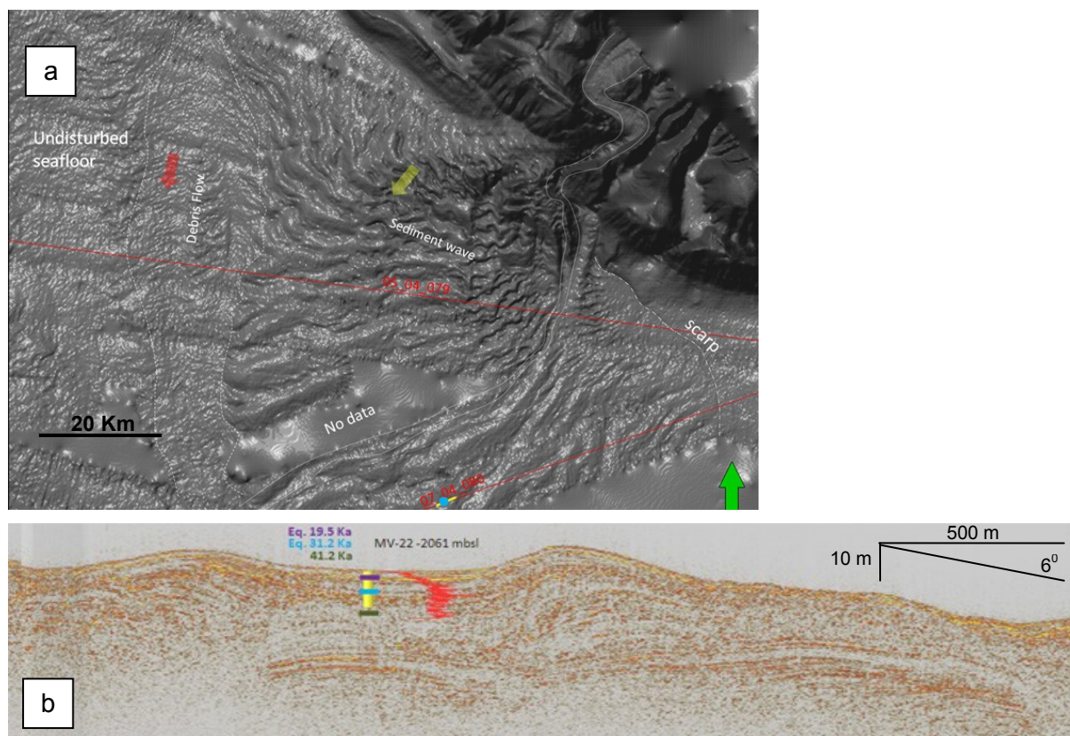
Figure 3: a) Gridded bathymetric data showing fan-shaped sediment waves observed in the Moresby Trough, with depositional dimensions of 2 km wavelength and 160-230 m height in the inner fan and 15-26 m in the outer fan. The origin of these depositional elements is interpreted as mass transport deposits overlain by thin turbidite layers.
