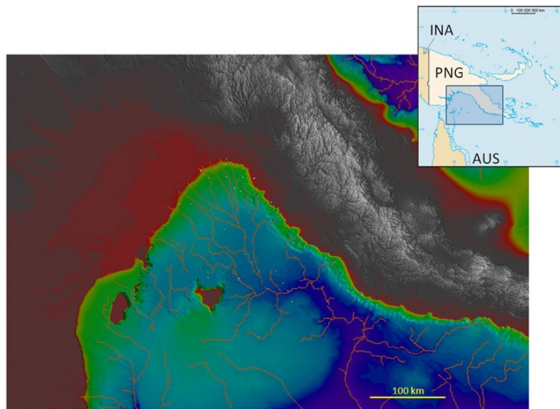
Figure 1: Topography and bathymetry of the Gulf of Papua (based on the DEM of Daniell, 2008), including major deepwater channel systems determined from slope analysis. Inset map showing study area location, AUS= Australia, INA= Indonesia, PNG= Papua New Guinea
