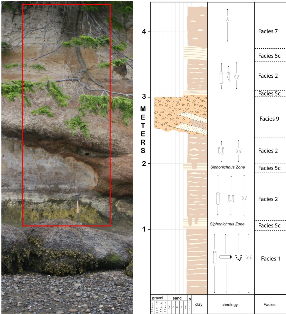
Figure 2: Example strip-log from Pleistocene outcrop. Red box (left photo) shows approximate location of strip log on outcrop. Strip log (right photo) shows the sedimentology (brown: mud; yellow: sand; orange: conglomerate), ichnological content and range, as well as where the individual units fit in the facies classification.
