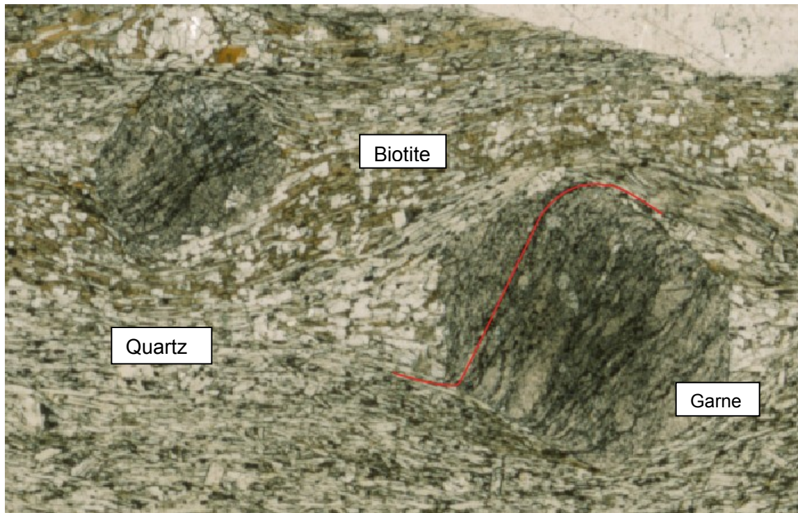
Figure 1: Sample G-16-D. Example of garnet with curved inclusion trails showing the relatively straight inclusions in the cores and curvature into the matrix foliation at the rim.
