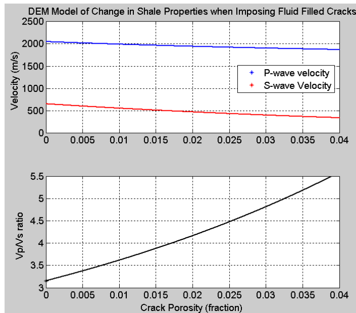
Figure 4: DEM modeling velocities for an increasing density of isolated and randomly oriented fluid filled cracks.
