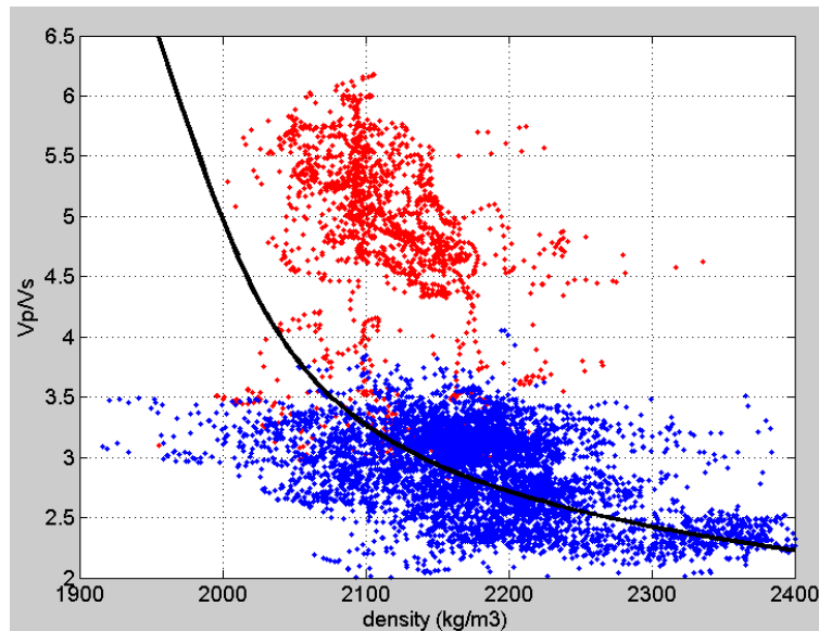
Figure 2: Vp/Vs trend for shales at Foster Creek. The trend line is from Vernik et. al. (2002). Red data correspond to wells in a region of anomalously low shear wave velocities.
