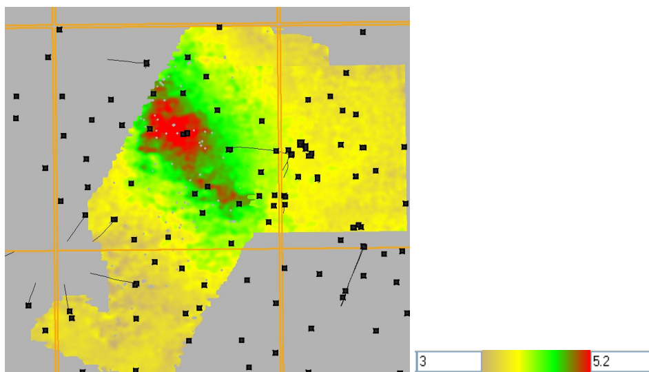
Figure 1: Colour represents V_p/V_s anomaly through the Lower Colorado Group. Section boundaries (1 mile interval) are shown.
