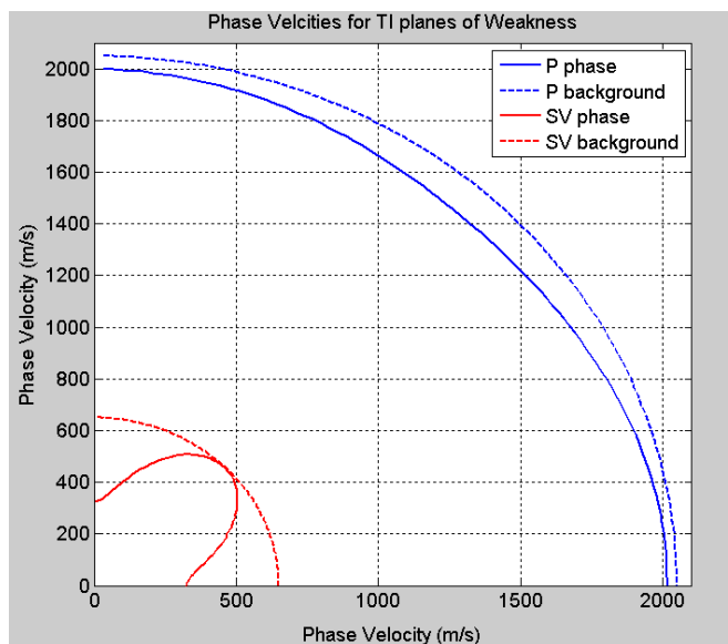
Figure 3: Phase velocities as a function of the angle from vertical for a series of horizontal planes of weakness described in the text. Dashed lines are isotropic velocities without cracks.
