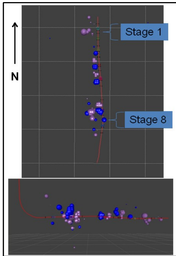
Figure 1. Map view and vertical cross-section through mapped locations of the microseismic events in this case study. Two types of microseismic events are color-coded: Blue spheres correspond to locations of the reverse faulting events and purple spheres correspond to locations of dip-slip events. Sphere size is proportional to the released seismic moment, the largest sphere (stage 8) represents 9.3 \cdot 10^9 Nm. Treatment well trajectory is represented by the red line. The induced events are predominantly located west of the treatment well. Dip-slip events are located at the depth of the treatment well while reverse mechanism show significant vertical growth.
