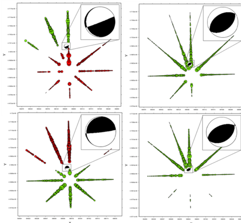
Figure 2 Map views of polarity and relative sizes of first arrivals for three types of microseismic events induced in this case study. Red circles represent motion down, green circles represent motion up, circles are proportional to relative sizes of the observed amplitudes. The black-and-white beach balls are plotted at the microseismic event epicenters as lower hemisphere projections of the inverted shear components of the general source mechanisms, with an enlarged beach ball in the upper right corner of each plot to show details of the failure mechanism.
