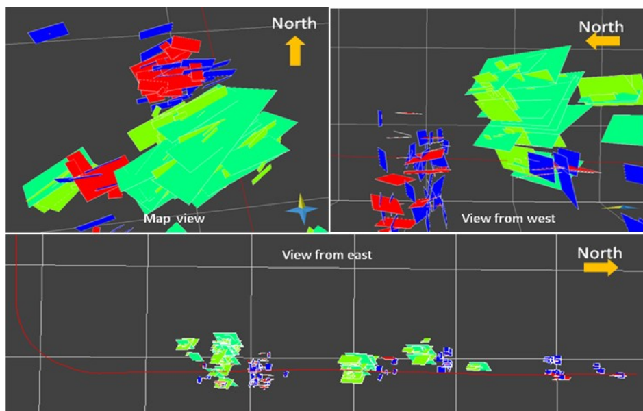
Figure 3: Discrete fracture network generated from microseismic event locations and inverted source mechanisms. Top left picture is a map view; green and turquoise colored fractures on the reverse failure mechanism planes. Right top picture shows vertical view looking from the west, displaying fracture planes representing the horizontal fractures (red) and associated dip slip fracture planes (blue). In bottom picture, fracture from all frac stages are displayed along the wellbore lateral; view is from the east.
