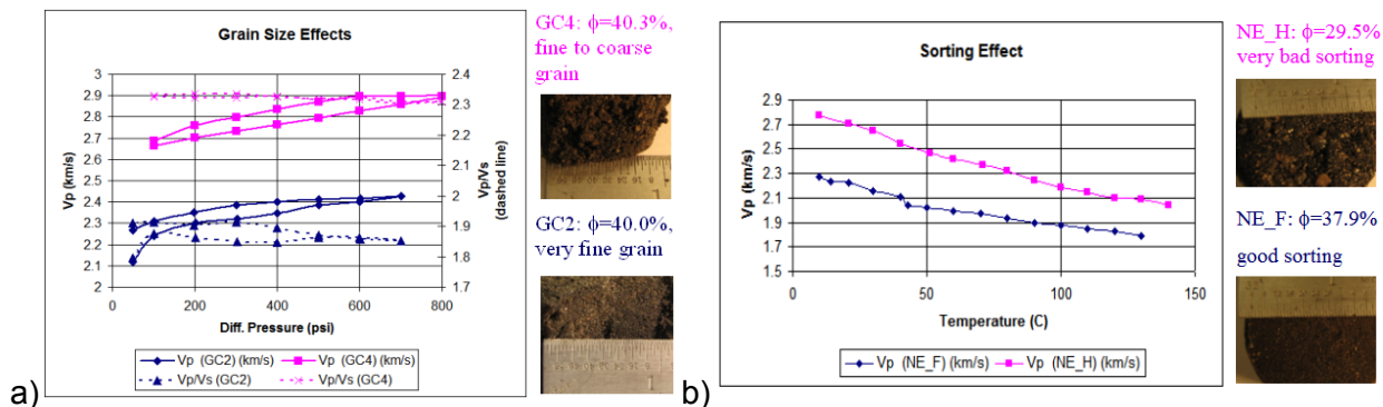
Figure 3 a) Grain size effect on velocity and Vp/Vs ratio for heavy oil sand samples; b) Grain sorting effect on velocity for heavy oil sand samples (Han et al., 2007)
