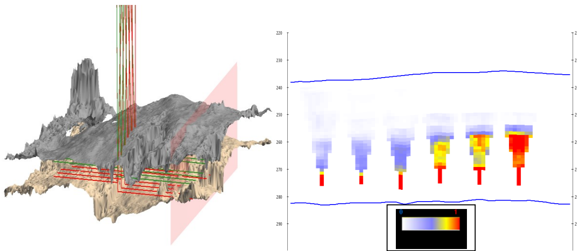
Figure 3: Left, proposed pads (producers in red, injector in green) between the median (P50) position of the top and base of the basal sands. Right, section going through the south pad (along the highlighted plane) after connectivity analysis.
