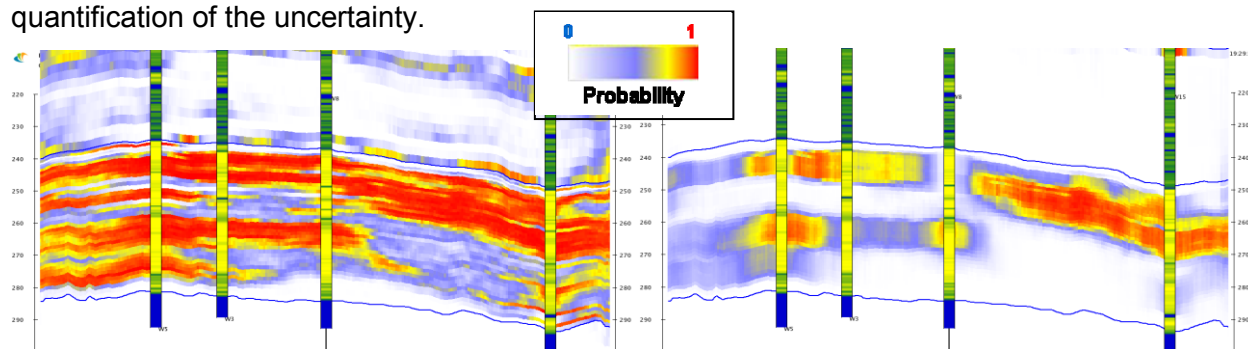
Figure 1: Bitumen probability (left) and thick continuous bitumen probability (right) in a random section (wells coloured by density, sands in yellow, shales in green and carbonates in blue)
