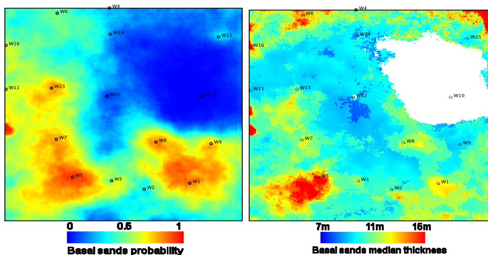
Figure 2: Map of probability of sands (left), map of P50 (median) of sands thickness (right). The white area has no basal sands.
