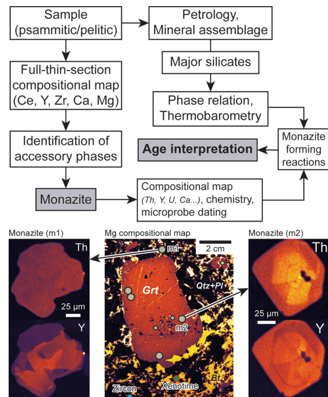
Figure 1: Flowchart of the approach, with example of a full-thin-section (cropped area) and two Y and Th compositional maps in selected monazite.
