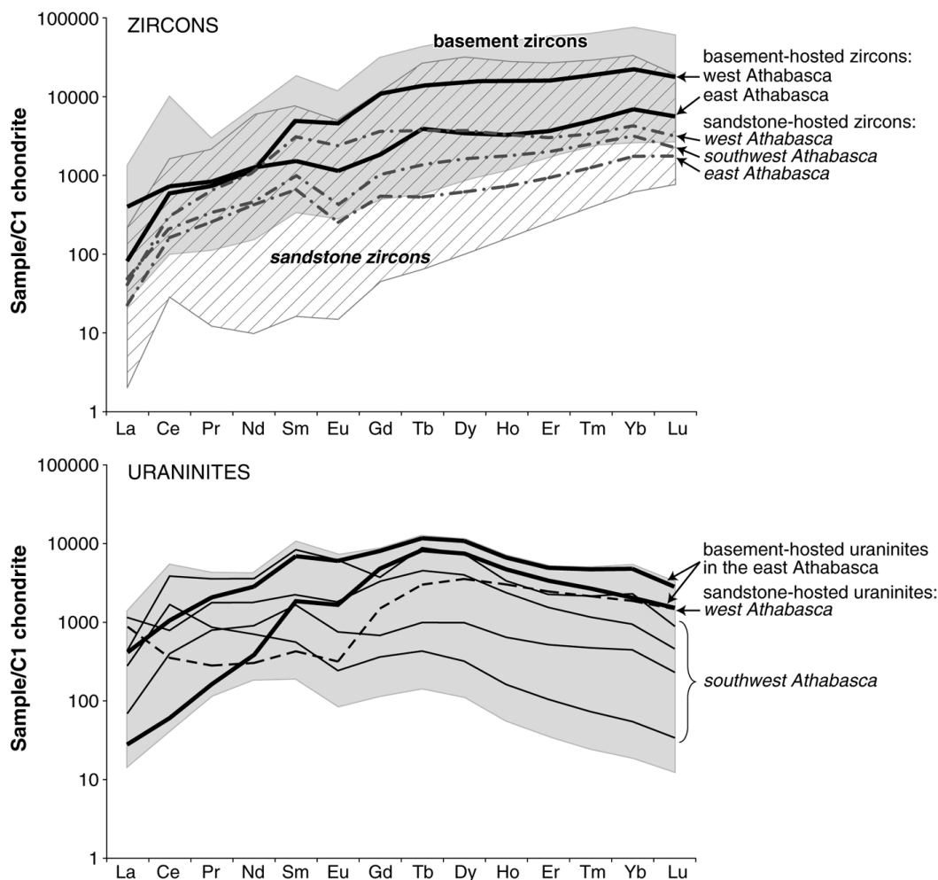
Figure 2. Rare Earth elements (REE) concentrations relative to C1 chondrite (McDonough and Sun, 1995) for zircons and uraninites from the Athabasca Basin. The gray and hatched areas represent the total variation fields for the minerals analyzed, whereas the lines represent the median values organized by location within the basin.
