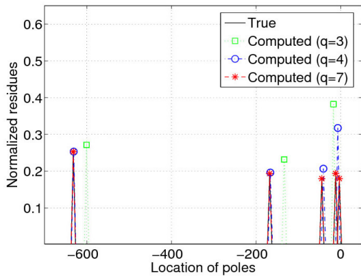
Figure 1 Reconstruction of residues and poles of the spectral function.
