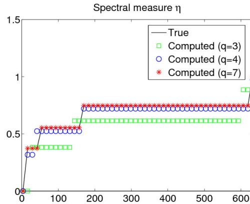
Figure 2 True and computed spectral measure.
