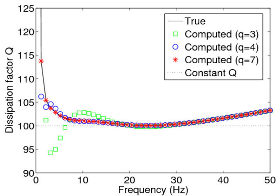
Figure 3 Reconstruction of the quality factor.
