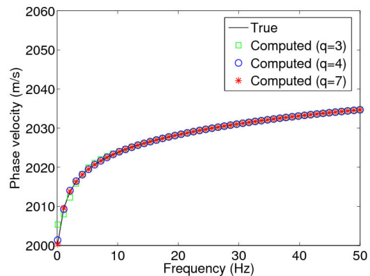
Figure 4 True and computed phase velocity.
