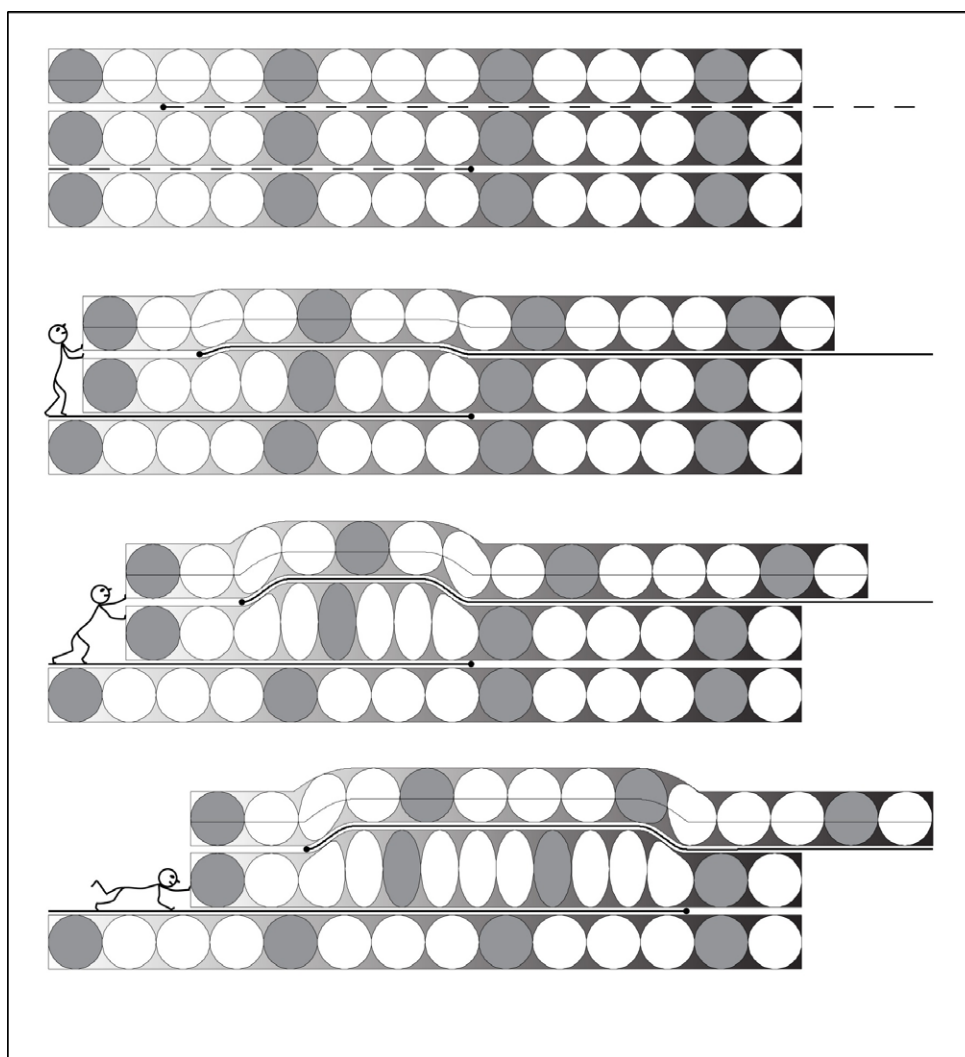
Figure 1: Deformation zone model. The four panels show a kinematic model as it develops increasing deformation. The upper panel shows the initial state with no deformation. The stick person shows displacement along the lower slip surface. Strain ellipses show the shortening and thickening within the middle unit. The upper unit slides on the upper slip surface and passively folds over the deformed middle unit.
