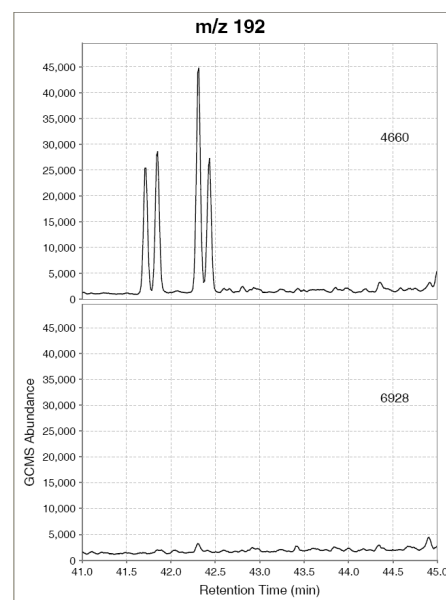
Figure 2: Mass chromatogram (m/z 192) showing severe biodegradation of methylphenanthrenes in sample #6928 (least biodegraded sample from AA/04-18-088-08W5/0) compared to a PROS standard oil.
