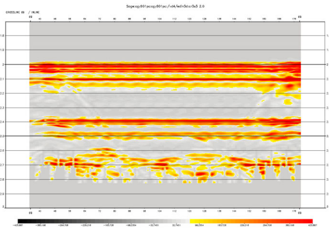
Figure 3: B^{\text{ani}} from NMO gathers.
