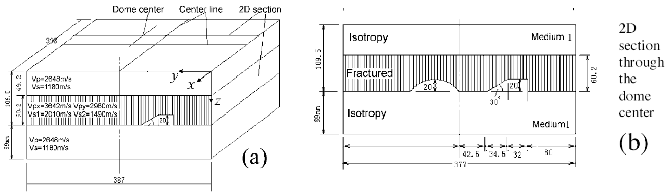
Figure 1: (a) 3D view of the model. (b) A 2D section through the center of the dome. There are two structures on the bottom of the fractured layer, a dome and a thrust fault. The modeling scale is 1:10,000. (After Wang and Li, 2003)
