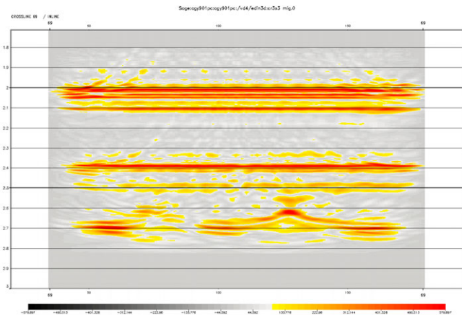
Figure 4: Post-stack migration of the B^{\text{ani}} result shown in Figure 3 (Zheng and Gray, 2002).
