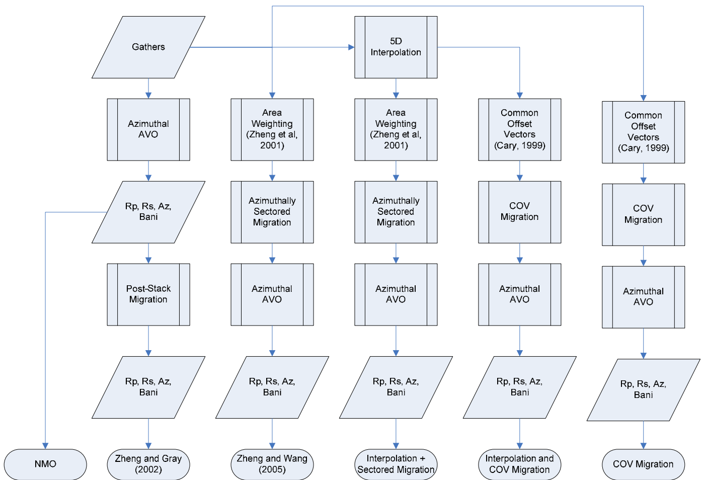
Figure 2: Flowchart showing the various azimuthal processing workflow tests.
