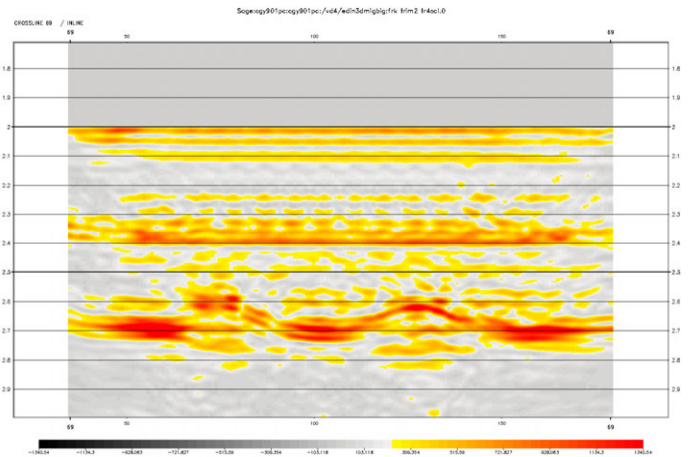
Figure 5: B^{\text{ani}} from azimuthally-sectored pre-stack migration with area-weighting (Zheng and Wang, 2005)
