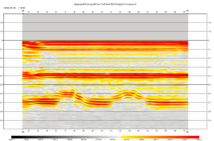
Figure 6: B^{\text{ani}} from azimuthally-sectored pre-stack migration with area-weighting after 5D interpolation of the gathers (Trad et al, 2005).
