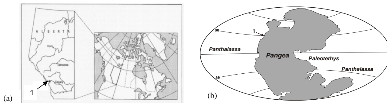
Figure 1: Location map (a) Kananaskis Country in southern Alberta, denoted by the number 1. (b) Paleolocation of study area on western margin of Pangea, denoted by the number 1. Modified from: Golonka, J., et. al., 1994.
