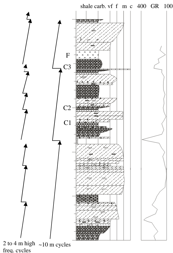
Figure 2: Stratigraphic Column with gamma ray log from Fortress Ridge Section, Kananaskis Country. Arrows indicate three ~10 m cycles along with higher frequency 2 to 4 m cycles. (vf, v, m, c refer to grain size). Conodont species of the genera Neognathodus and Idiognathodus from samples C1 and C2 indicate correlation with lowermost Moscovian (Verean substage) or Lower Atokan (USA). Conodonts from C3 and the fusulinacean (F) Profusulinella fittsi are consistent with the second substage of the Moscovian (Kashirian) or mid-Atokan (USA).
