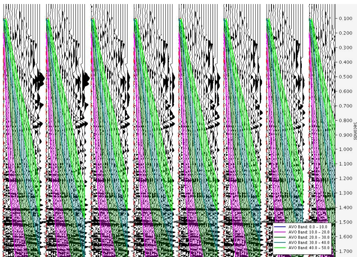
Figure 3 shows migrated gathers with angles overlaid. Residual flattening of the gathers is necessary in order to successfully invert the data.
