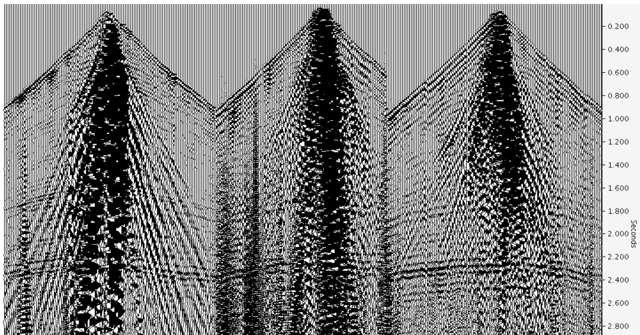
Figure 1 shows a selection of shots from a single survey. The variable noise content will affect the stability of the deconvolution operators.
