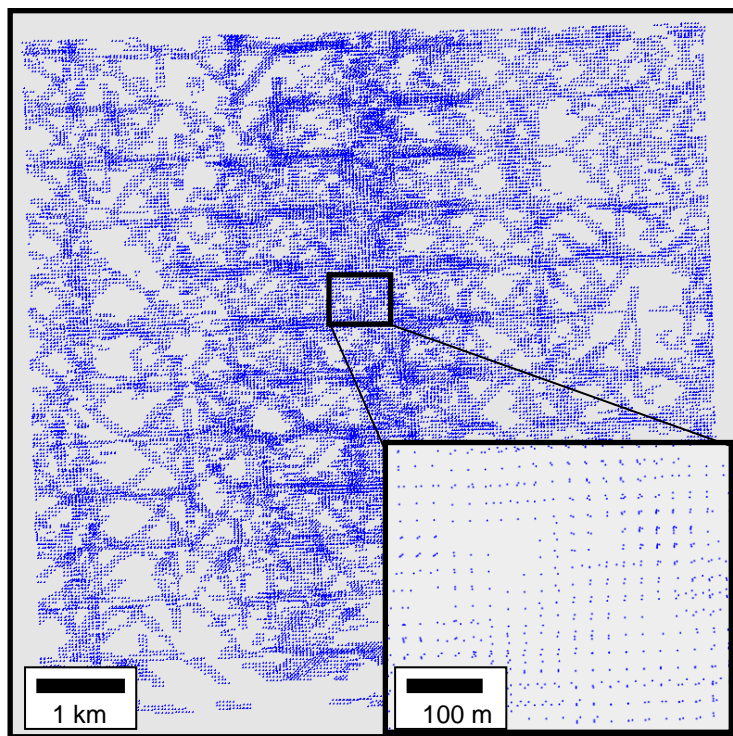
Figure 3: Midpoint coordinates in an overlap zone between two 3D seismic surveys with offsets ranging from 1200 – 1350 m. The irregular sampling needs to be considered in order to minimize artifacts in a Kirchhoff migration pre-stack-time migration.
