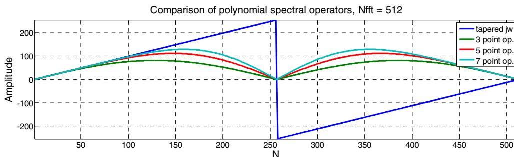
Figure 4 Comparison of the amplitude spectra for polynomial derived operators for operator sizes 3, 5, and 7 points.
